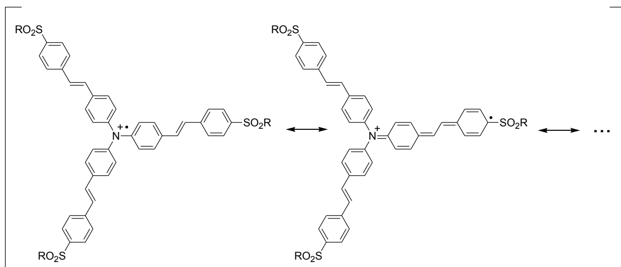
SCHEME 3: Stabilization of the radical cation of the octupolar derivatives.
