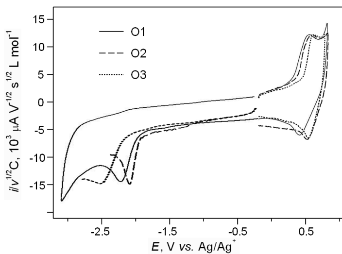
Figure 4. Normalized voltammograms of compounds O1-O3 at a GC disk electrode in 0.1 M Bu 4 NPF 6 solution in THF/CH 3 CN (5:1 v/v). Scan rate \nu = 1 \text{ V s}^{-1} .
