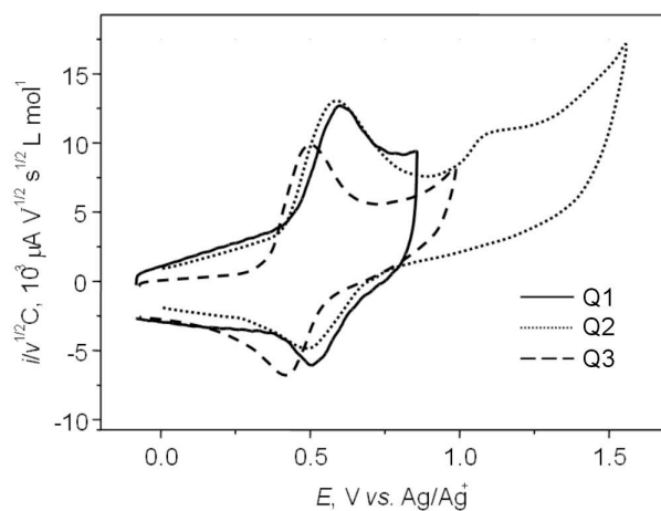
Figure 3. Normalized voltammograms of oxidation of compounds Q1-Q3 (respectively D- \pi -D, D- \pi -D' and D'- \pi -D') at a gold disk electrode in 0.1 M Bu 4 NPF 6 solutions in THF/CH 3 CN (3-5:1 v/v). Scan rates for Q1-Q3 , respectively: \nu = 0.1, 2.5, 2.5 \text{ V s}^{-1} .
