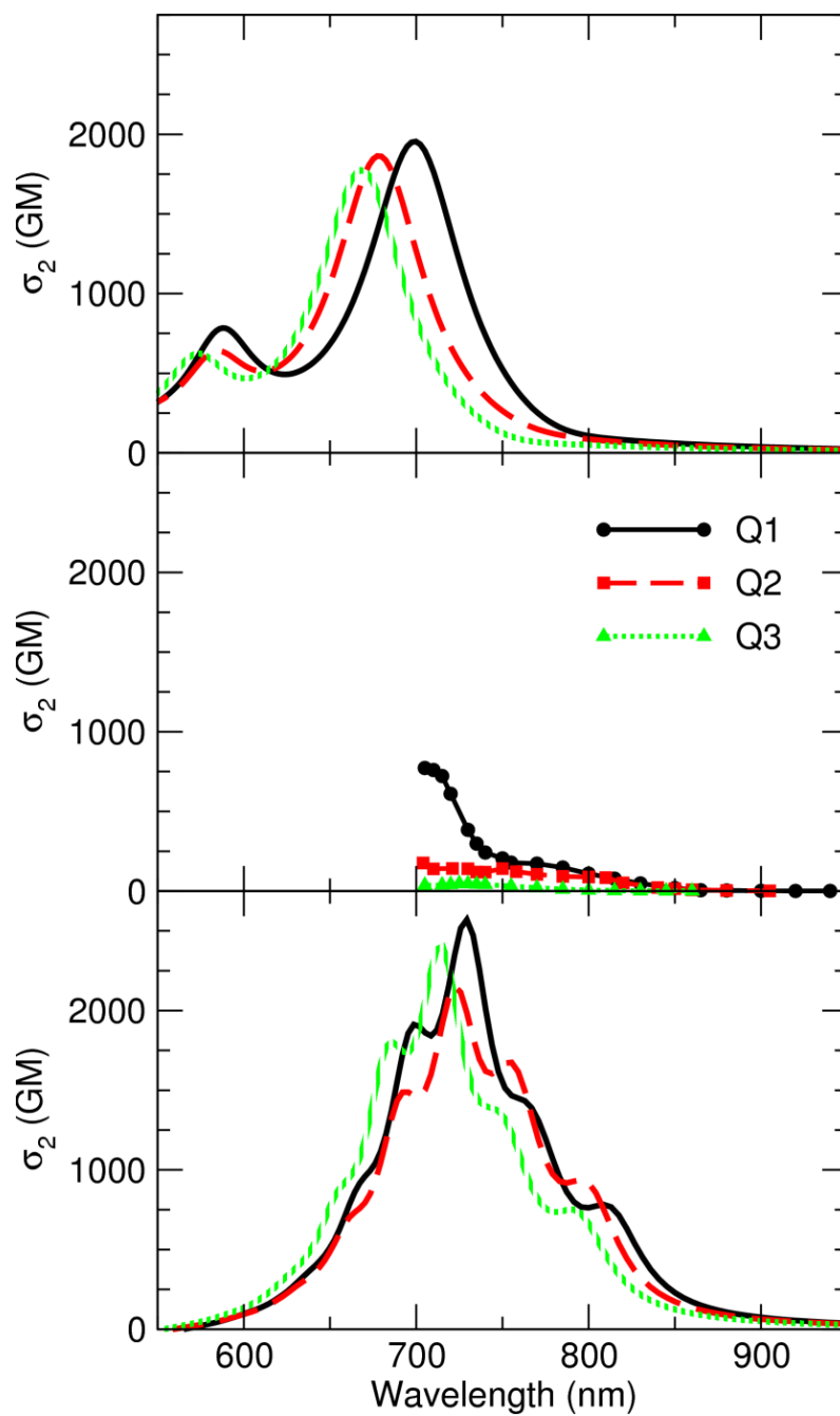
Figure 11. Two-Photon absorption cross-section for quadrupoles Q1-Q3 : TD-B3LYP calculated data in vacuum (top), experimental data in toluene (middle) and spectra calculated through essential-state models for \epsilon_{or} = 0 (bottom, see parameters in Figure 5).
