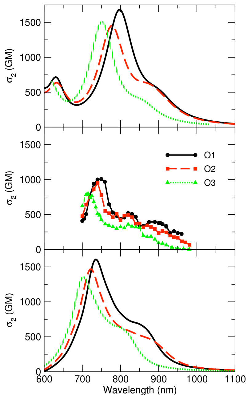
Figure 12. Two-Photon absorption cross-section of octupoles O1-O3 : TD-B3LYP calculated data in vacuum (top), experimental data in ethanol (middle) and spectra calculated through essential-state models for \epsilon_{or} = 0.2 (bottom, see parameters in Figure 6).
