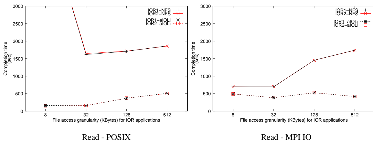
Figure 7: Impact of an I/O intensive application on a second one
