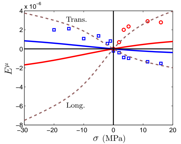
Fig. 11. \Delta E effect for Ni-Zn ferrite: longitudinal and transverse magnetostriction strain as a function of the applied stress \sigma , modeling (line) and experimental results. Dashed lines: Results obtained with a full multiscale model [12].
