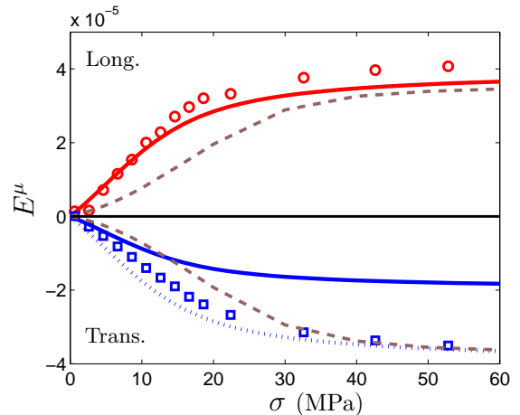
Fig. 13. \Delta E effect for an iron-cobalt alloy: longitudinal and transverse magnetostriction strain as a function of the applied stress \sigma , modeling (line) and experimental (points) results. Plain line for isotropic strain and dot line (transverse direction) for configuration energy effect. Dashed lines: Results obtained with a full multiscale model with configuration energy effect [5, 15, 16].
