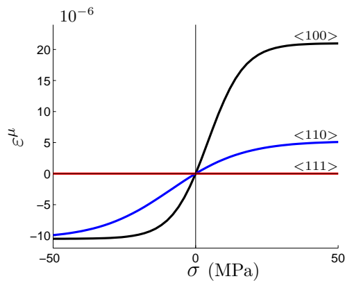
Fig. 3. \Delta E effect in the case of iron single crystal.
