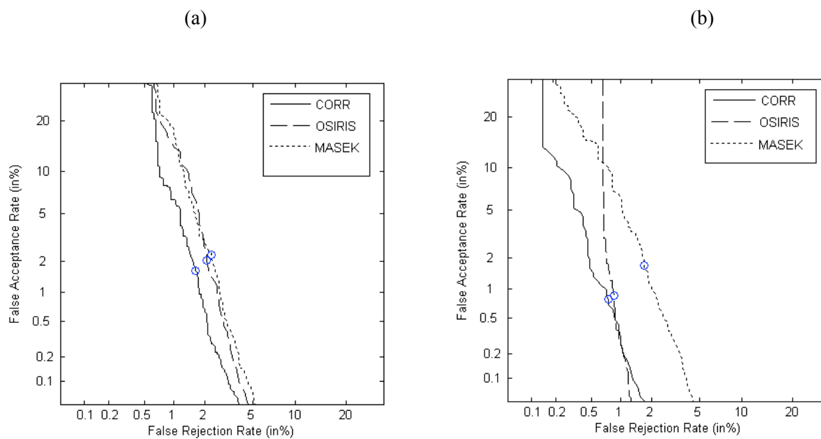
Fig.6 DET curves of CORR system (solid curve), OSIRIS system (dashed curve) and MASEK (dotted curve) on: (a) Bad and average quality subset (quality 3: 18 images and quality 4: 392 images), (b) Good quality subset (quality 5: 1015 images), of
