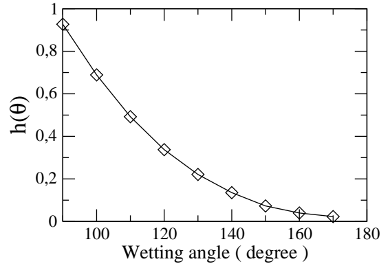
FIG. 2: Numerical values obtained for h(\theta) .
