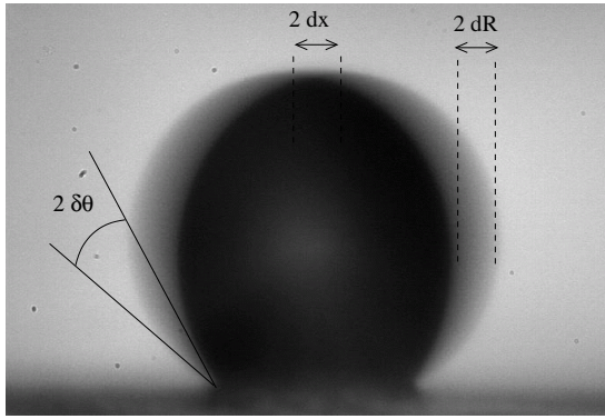
FIG. 5: Image of a vibrating R = 0.192\text{mm} mercury drop. The measure of the ghost radius variation dR permits to calculate both \delta\theta and dx .
