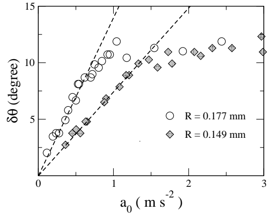
FIG. 8: Maximum wetting angle variation \delta\theta as a function of the and 0.
