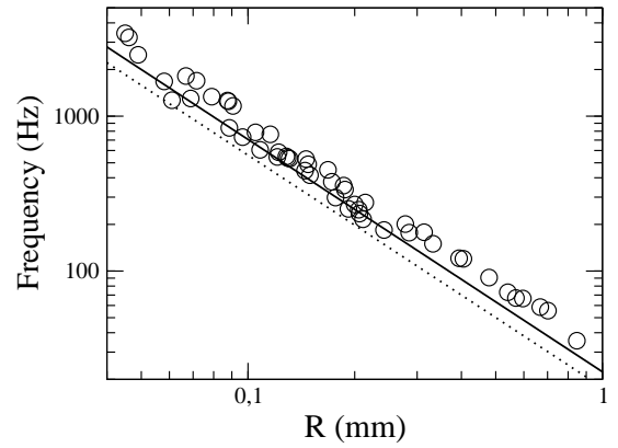
FIG. 6: Eigen frequency as a function of the drop size. The dotted and full lines are calculated using Equ. 6 respectively v
