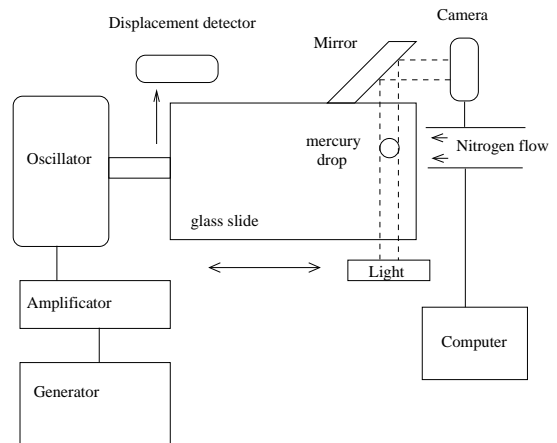
FIG. 4: Schematic representation of the experimental apparatus.
