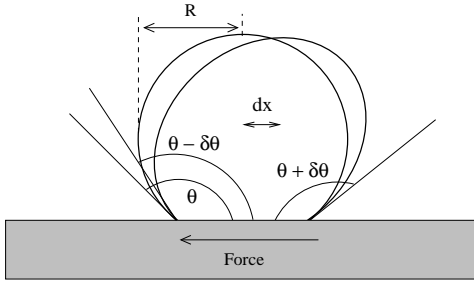
FIG. 1: Schematic representation of the droplet shape under the influence of an external force. The deformation induces a displacement dx of the center of mass and a variation \delta\theta of the advancing and receding wetting angles.
