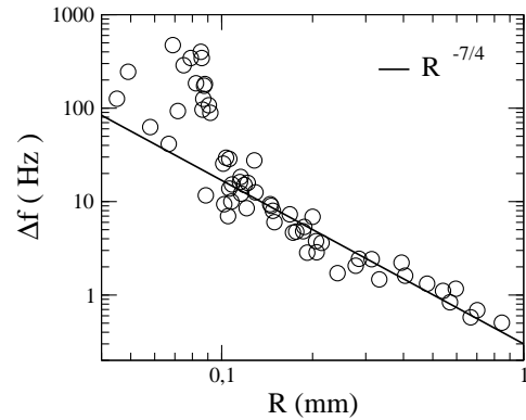
FIG. 9: Inverse of the relaxation time \alpha as a function of the droplet radius. The full line represent the best fit to the expected scaling law (Equ. 9) for the larger droplet sizes.
