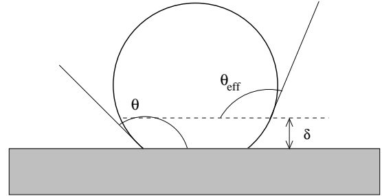
FIG. 3: Schematic representation of the effective wetting angle associated to the Stoke length.
