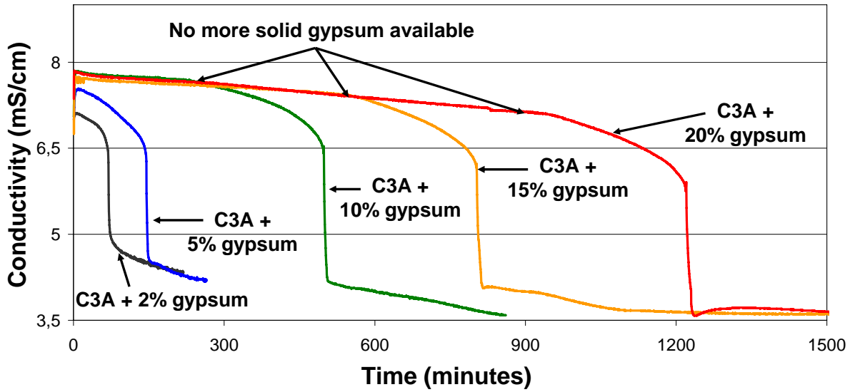
Figure 7. C3A hydration in limewater with various calcium sulphate weight ratio: conductivity curves (various amount of gypsum, L/S = 20, [Ca(OH) 2 ]=20mM).
