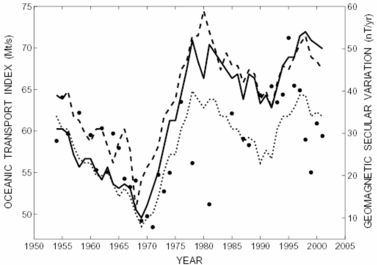
The relationship of the oceanic transport index of the North Atlantic gyre circulation and geomagnetic index variation
