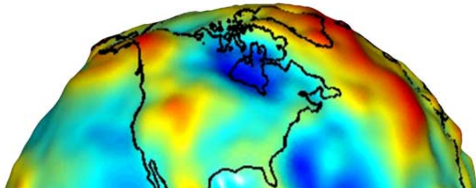
Earth's Gravity Field Anomalies (milligals)
