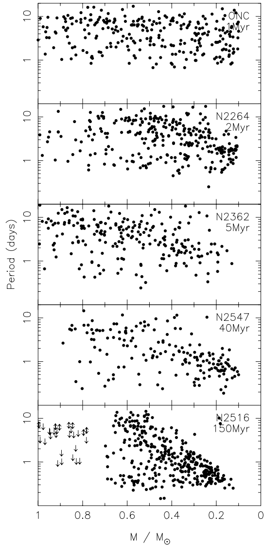
Figure 12. Rotation period as a function of stellar mass for (top to bottom): ONC, NGC 2264, 2362, 2547 and 2516. Lower and upper limits (from v \sin i data) are marked with arrows. The masses were taken from the NEXTGEN mass–magnitude relations (Baraffe et al. 1998) at the appropriate ages. The ONC data are from Herbst et al. (2002). For NGC 2264 we used the data of Lamm et al. (2005) and Makidon et al. (2004). The NGC 2547 and 2516 rotation period data are from the Monitor project (Irwin et al. 2007b,c).
