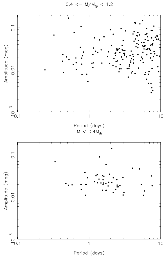
Figure 10. Plot of amplitude as a function of period for NGC 2362 in two mass bins: 0.4 \leq M/M_\odot < 1.2 (top) and M < 0.4 M_\odot (bottom).
