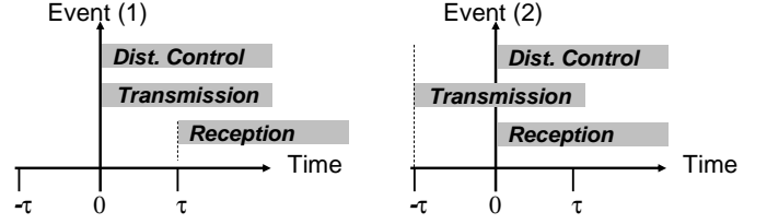
Fig. 1. Protocols to ensure that the agents reach the average of the initial position
