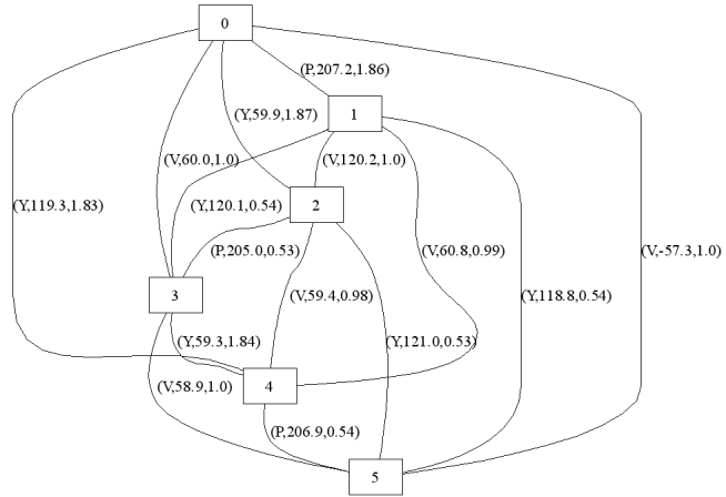
Fig. 5. Associated topological graph
