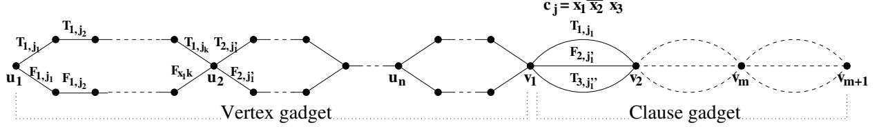
Figure 6: Reduction of Maximum 3 Satisfiability to MC- st -Path with colors of span 2
