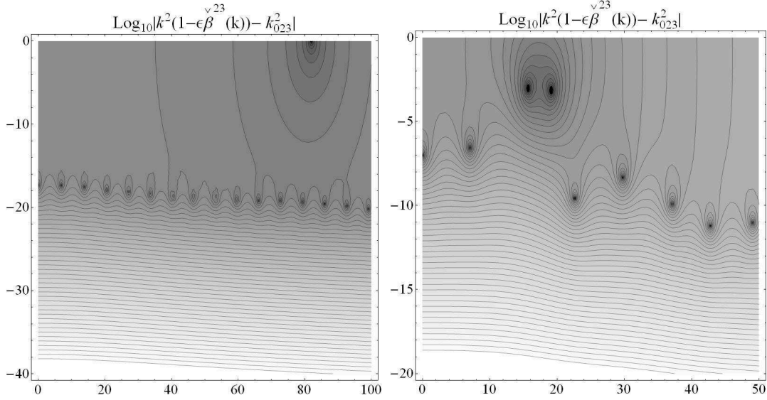
Figure 2: Contour plots of |k^2(1-\epsilon\check{\beta}^{\check{m}n}(k))-k_{0mn}^2| in the mode m = 2, n = 3 . Aluminium plate in contact with air \epsilon \approx 0.005 (left) and water \epsilon \approx 4.5 (right).
