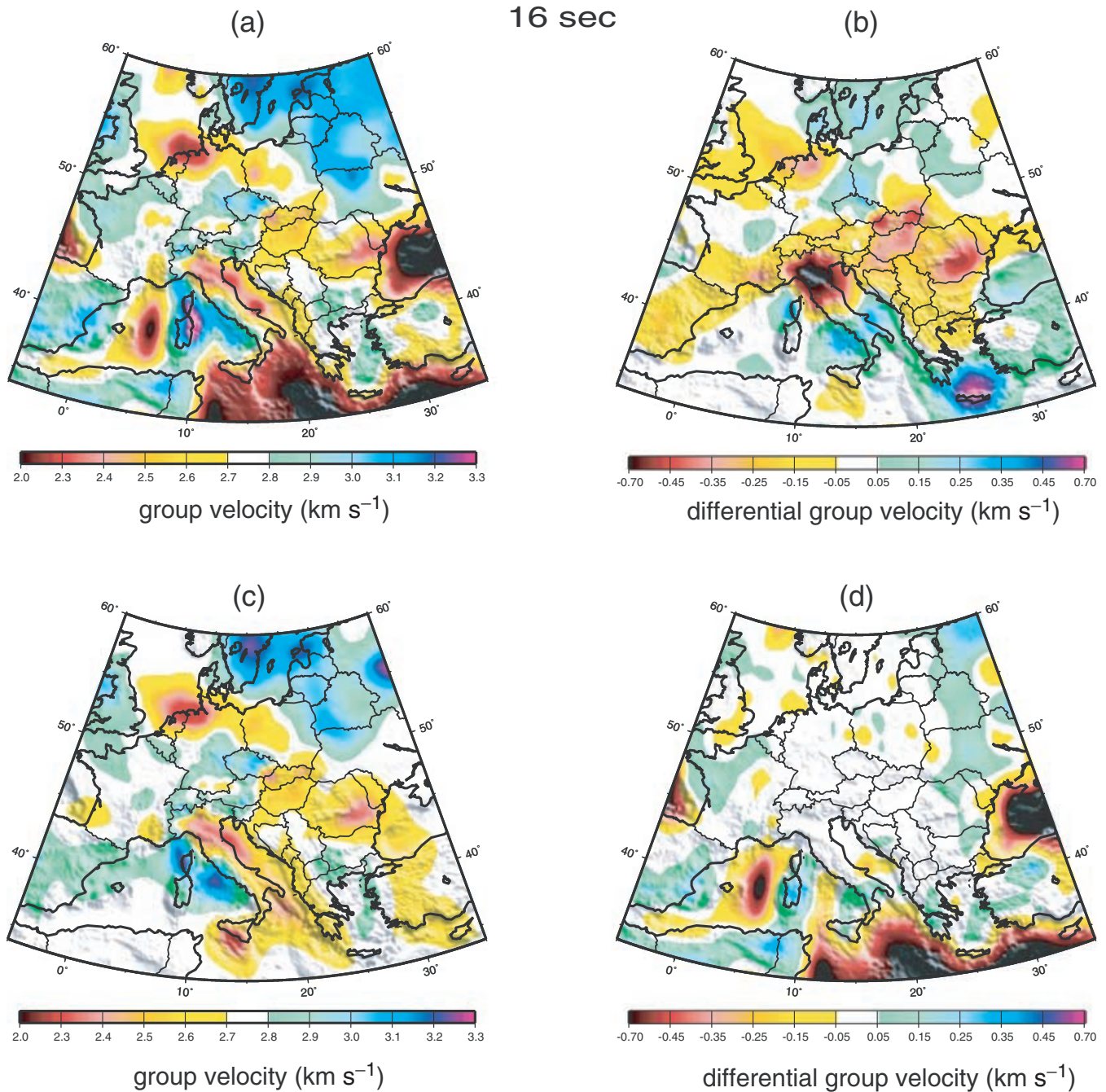
Figure 10. Group speed maps at 16 s period. (a) Estimated group speed map determined with a reference map. (b) Difference between the estimated map in (a) and the reference map presented in Fig. 12(a). (c) Estimated group speed map determined without a reference map. (d) Difference between the two estimated maps in (a) and (c).
