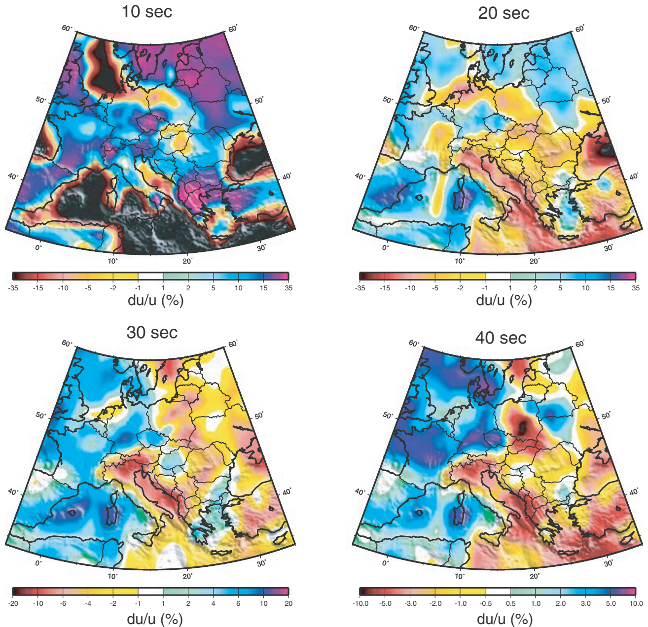
Figure 9. Estimated group speed maps at 10, 20, 30 and 40 s periods. Maps are presented as a perturbation from the average across the map in per cent.
