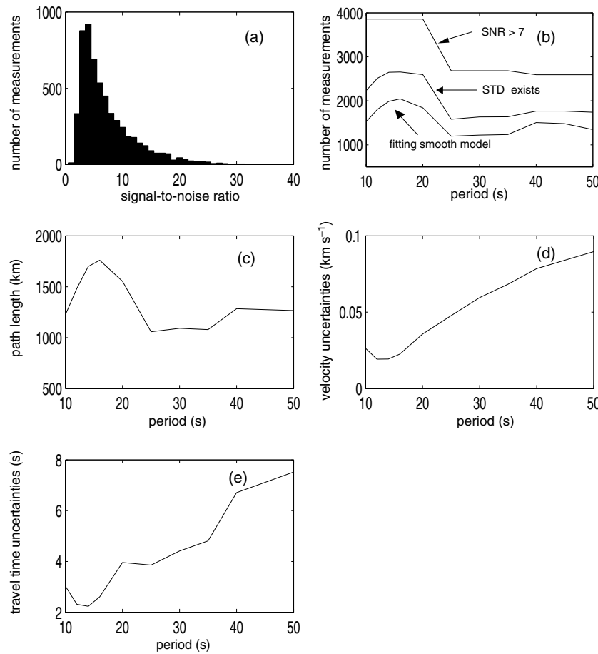
Figure 5. (a) Number of measurements versus SNR from the 12 month stacked cross-correlations. (b) Number of measurements remaining after several steps in data reduction. (c) Average path length of the accepted dispersion measurements. (d) Average group speed uncertainties versus period. (e) Average traveltime uncertainties versus period.
