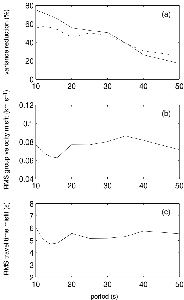
Figure 13. Various misfit statistics for the estimated group speed maps to the observations taken after all stages of data rejection are complete. (a) Misfit is presented as reduction of variance delivered by the estimated maps relative to (solid line) the predicted group velocity maps from the global 3-D model (Shapiro & Ritzwoller 2002) and (dashed line) the average velocity across each map. (b) rms group velocity misfit presented versus period. (c) rms traveltimes misfit presented versus period.
