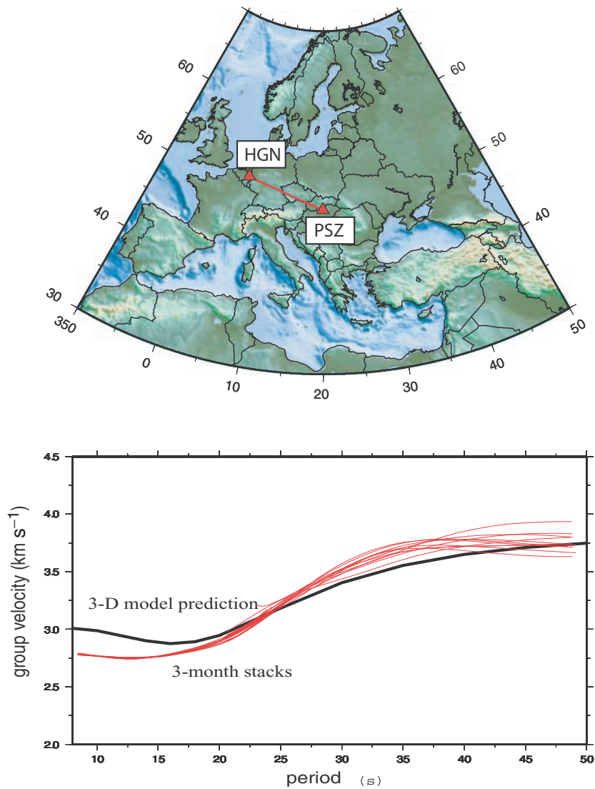
Figure 6. An example of seasonal variability of the dispersion measurements. Top: the path considered is between stations HGN (Heijmans Groeve, Netherlands) and PSZ (Piszkes-teto, Hungary). Bottom: the red curves are group velocity measurements obtained on twelve 3 month cross-correlations bandpass filtered from 8 to 50 s period. The black line is the prediction from the global 3-D model (Shapiro & Ritzwoller 2002).
