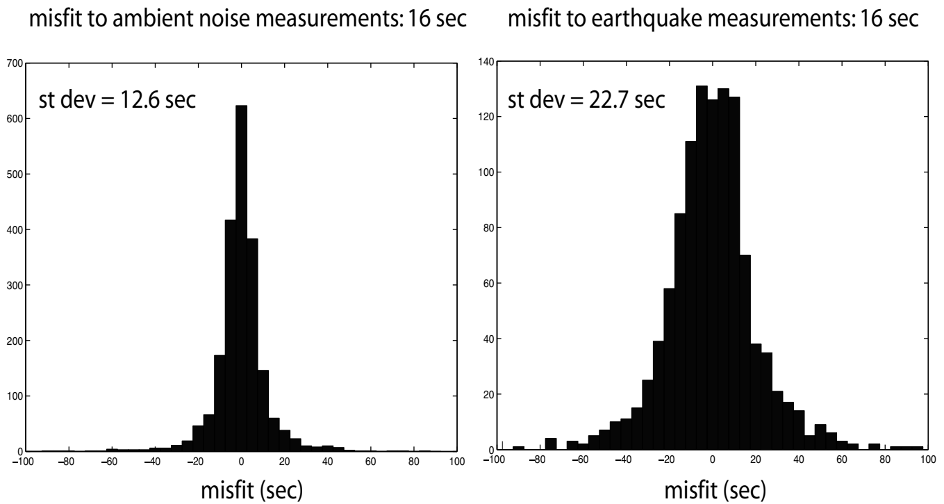
Figure 7. Histograms of misfit for ambient noise data (left) and earthquake data (right) at 16 s period. Misfit is calculated from the corresponding oversmooth tomographic map inverted from ambient noise data and earthquake data. Ambient noise data are taken prior to the stage where measurements are rejected due to large misfit. The standard deviation is shown at the left top of each diagram.
