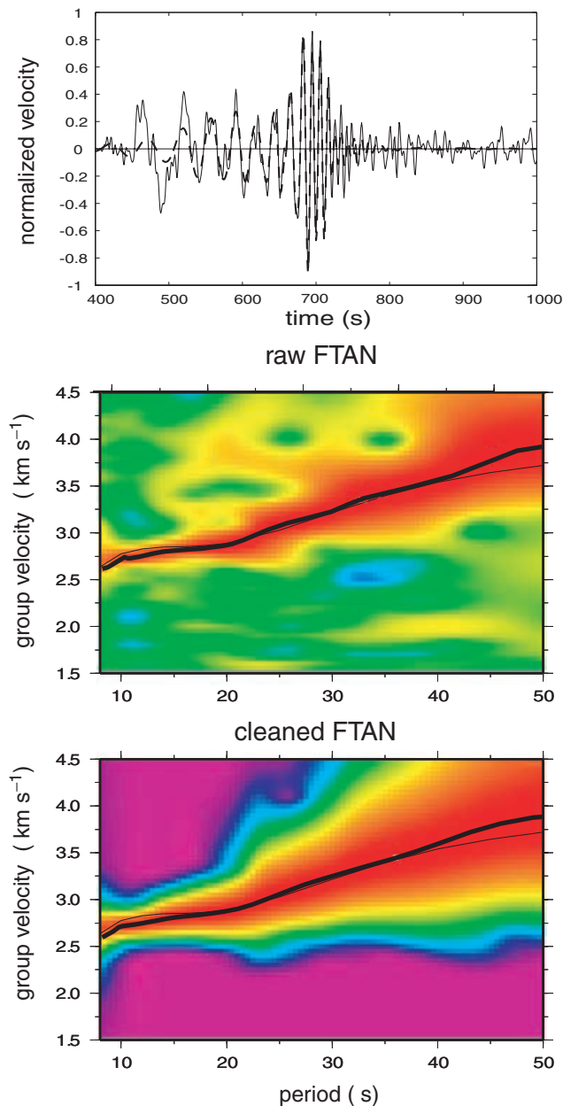
Figure 4. Example of dispersion measurement. Top: 1 yr symmetric component cross-correlation obtained between stations IBBN (Ibbenbueren, Germany) and OBN (Obninsk, Russia), which are separated by 1900 km. Middle: raw frequency time (FTAN) diagram in which the thick line is the raw dispersion measurement. Bottom: cleaned FTAN diagram obtained after applying the phase-matched filter based on the raw dispersion measurement. The thin line in the middle and bottom panels is the dispersion curve predicted from the global 3-D shear velocity model (Shapiro & Ritzwoller 2002). The cleaned waveform is overplotted in the top panel as a dashed line.
