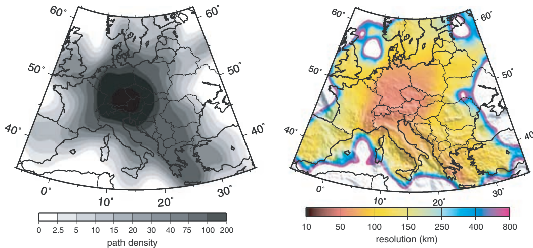
Figure 8. Path density (left column) and resolution estimates (right column) at 16 s period. Path density is defined as the number of rays intersecting a 1^\circ \times 1^\circ ( 111 \times 111 \text{ km}^2 ) square cell. Resolution is presented in units of km, and is defined as the standard deviation of a 2-D Gaussian fit to the resolution surface at each model node.
