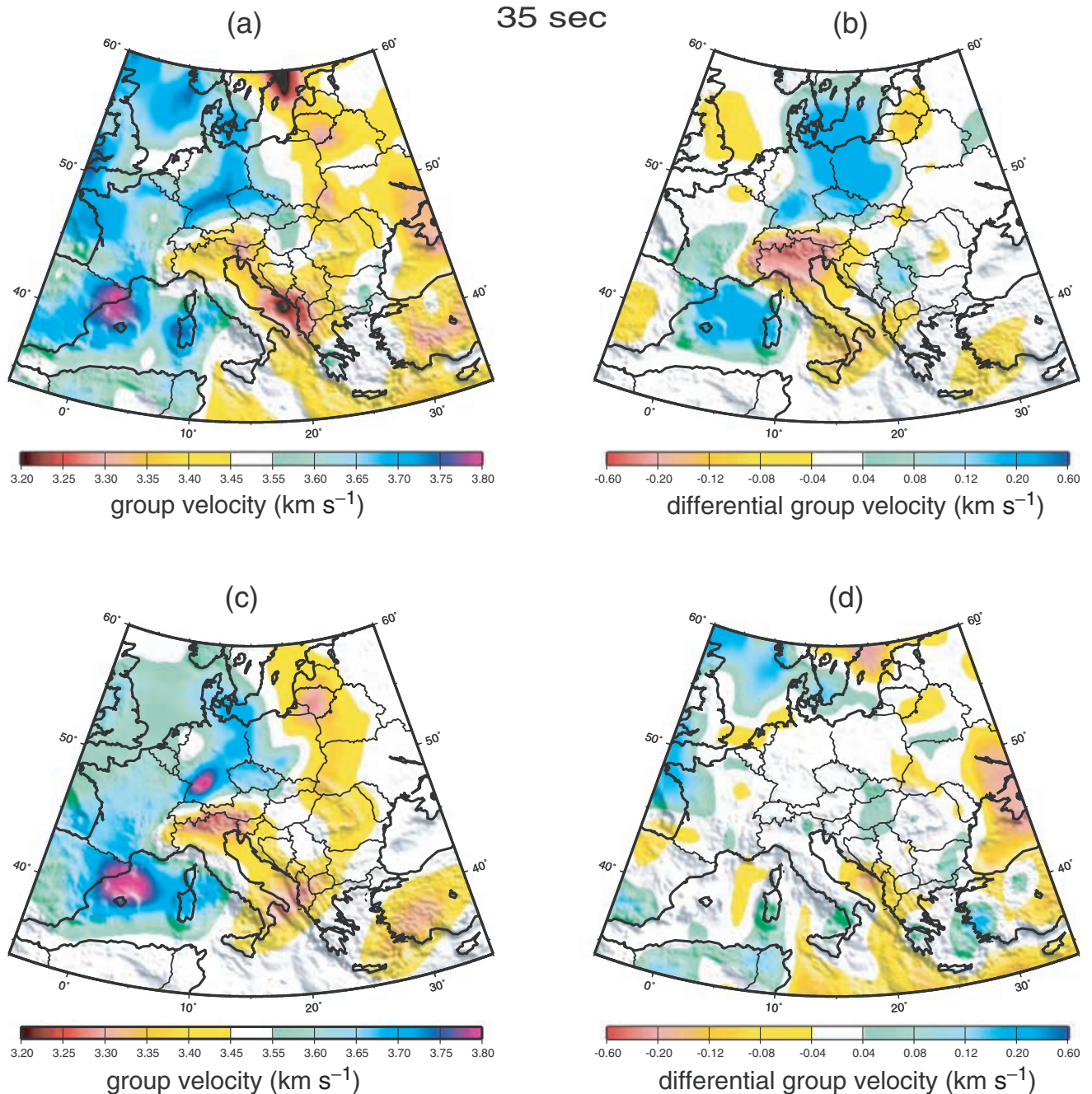
Figure 11. Same as Fig. 10, but for 35 s period. The reference map used is presented in Fig. 12(b).
