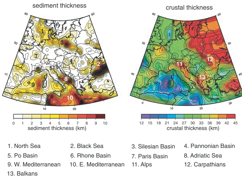
Figure 15. Maps of sediment thickness (left) and crustal thickness (right). Sediment thicknesses are taken from CRUST1.0, which Laske and Masters digitized across most of Europe from the EXXON Tectonic Map of the World. Crustal thicknesses are taken from CRUST2.0. The locations of geological units discussed in the text are marked approximately.
