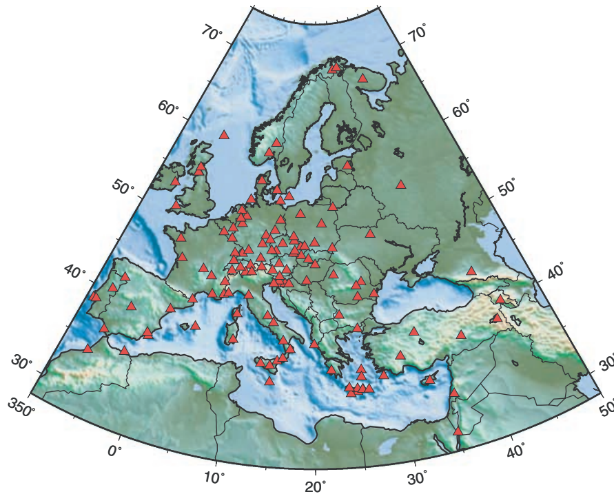
Figure 1. Broad-band seismic stations in Europe used in this study, marked by red triangles.
