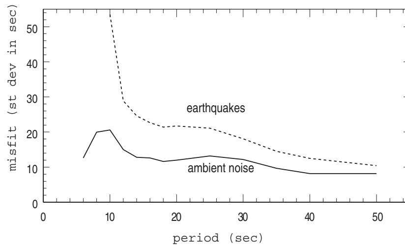
Figure 14. Standard deviations of data misfit after tomography with an oversmoothed model, presented as a function of period for ambient noise data (solid line) and earthquake data (dashed line). In contrast with Fig. 13(c) and similarly to Fig. 7, the last stage of data rejection has not been applied here.
