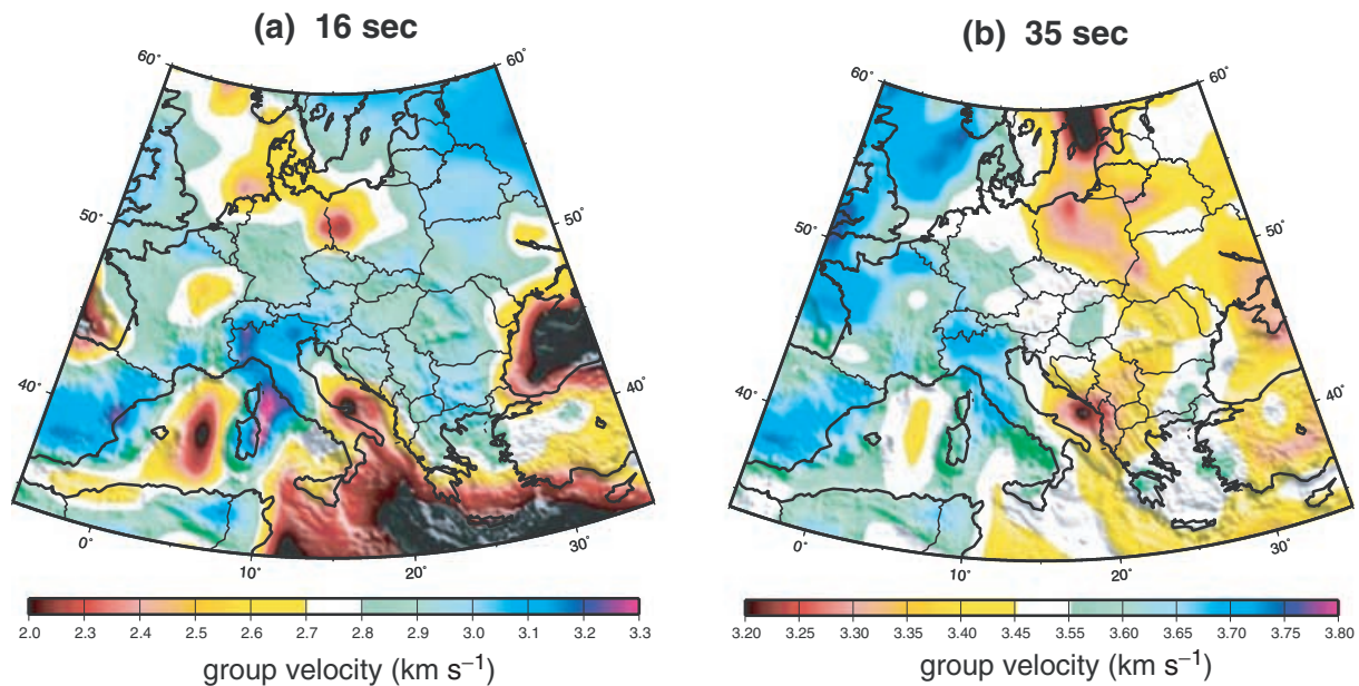
Figure 12. Reference maps computed from the 3-D model of Shapiro & Ritzwoller (2002) at (a) 16 s and (b) 35 s period.
