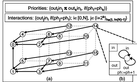
Fig. 7. The Parallel Adder
