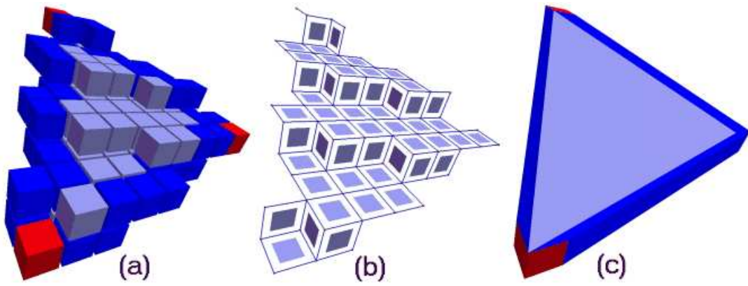
Fig. 8. Standard triangle with (a) Voxel view (b) Cell-complex view (c) Analytical view
