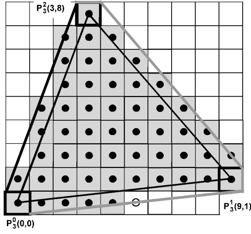
Fig. 7. Standard cover of a 2D triangle
