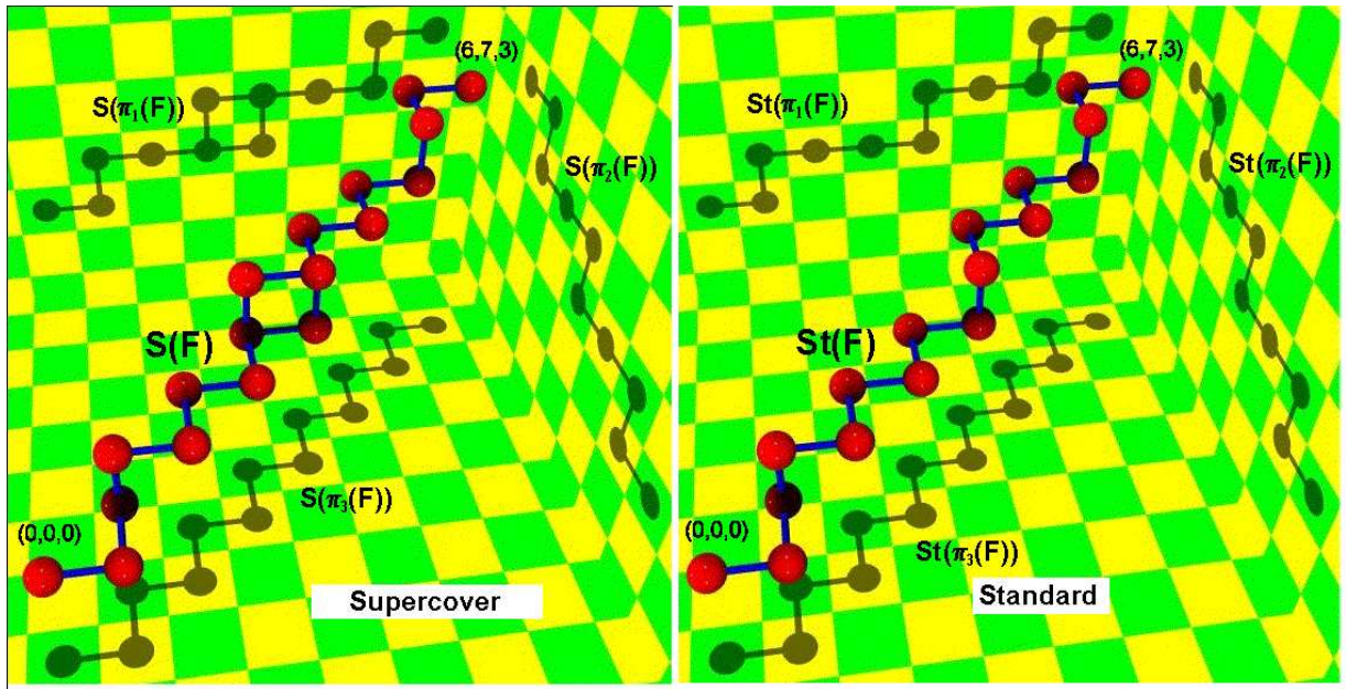
Fig. 6. Supercover and Standard 3D line.
