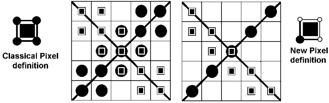
Fig. 3. Supercover discretisation of x_1 - x_2 = 0 and x_1 + x_2 = 0 with classical and modified pixel definition.
