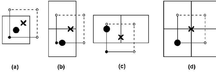
Fig. 5. Different configurations of 2D standard points. A standard point is formed of only one discrete point.
