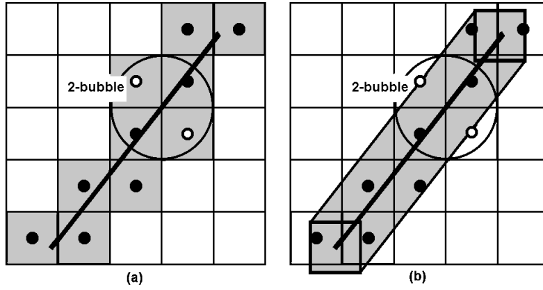
Fig. 2. Supercover definitions.
