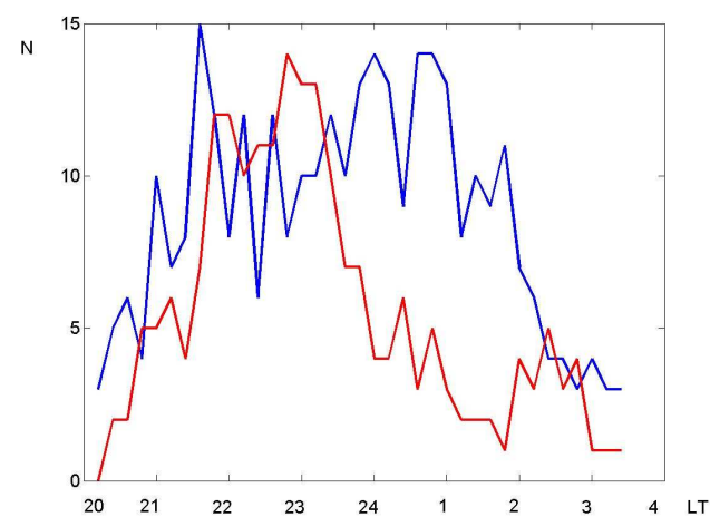
Fig. 1. Number of Es-spread observations as function of the local time LT for “background” days (blue) and “seismoactive” (−2,−1,0) days (red).
