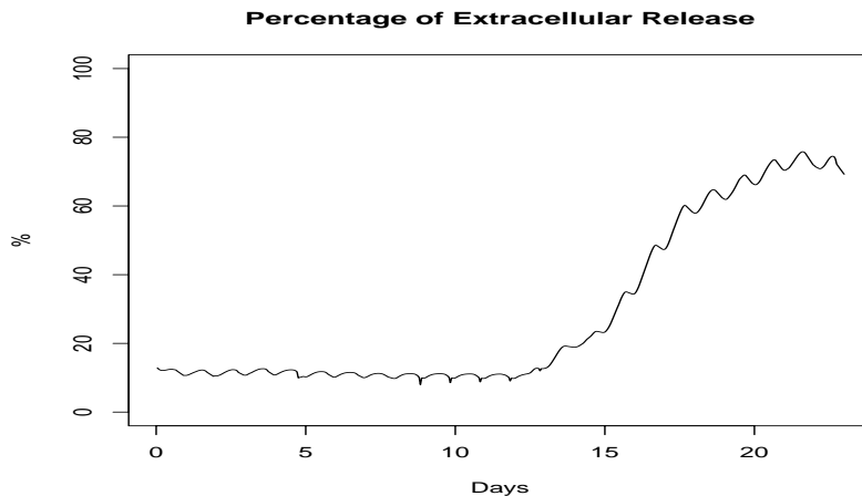
Fig. 8. Percent of DOC excretion compared to total organic carbon produced by Emiliania huxleyi .
