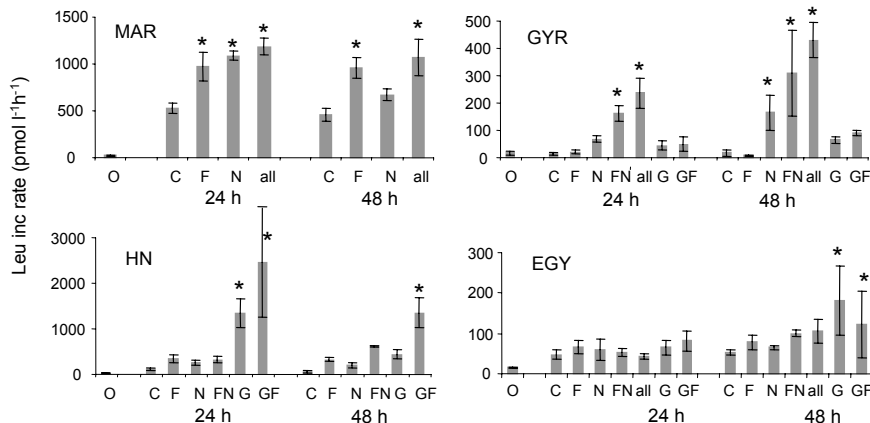
Fig. 2. Evolution of leucine incorporation rates on bioassay experiments made under “trace metal clan” conditions. Means ± sd of triplicate bottles sampled after 24 and 48 h of incubations. For MAR and HNL enrichments were O: initial conditions, C: control nonenriched, F: +iron, N: + nitrates+ammonium+phosphates+silicates, all: nitrates+phosphates+silicates+iron, G: +glucose, GF: glucose + iron. For GYR and EGYR N was only nitrate+ammonium, FN was nitrate+ammonium+iron and all nitrates+ammonium+phosphates +iron. *: response significantly different from the control at the same time, ANOVA test, p < 0.05.
