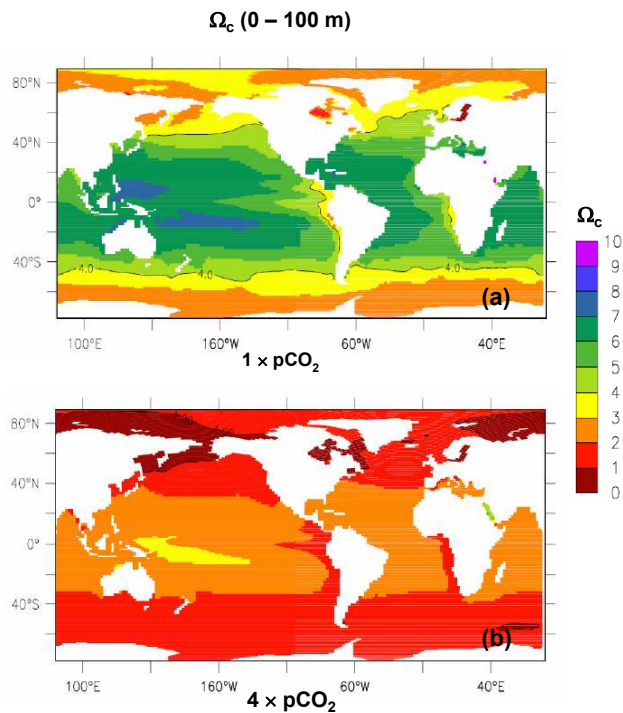
Fig. 4. Saturation state \Omega_c of surface ocean (0–100 m): (a) 1x pCO 2 and (b) 4x pCO 2 .
