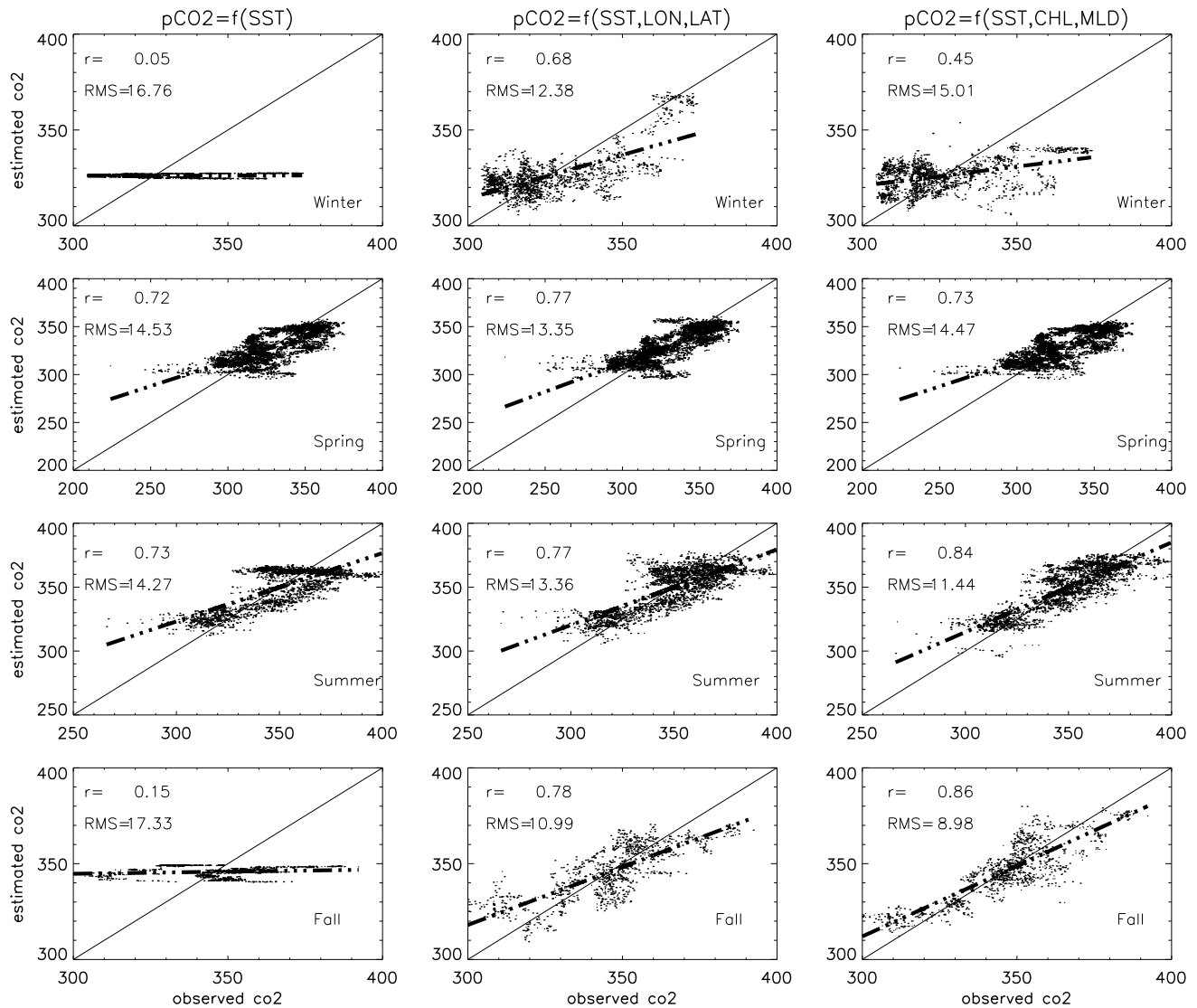
Fig. 2. Scatterplots of the in-situ pCO 2 vs. estimated pCO 2 obtained by three linear regressions based on the training data set: Left column pCO_2=f(SST) (Eq. 2); middle column: pCO_2=f(SST, \text{longitude}, \text{latitude}) (Eq. 4), right column: f(SST, CHL, MLD) (Eq. 3) for winter, spring, summer and fall.
