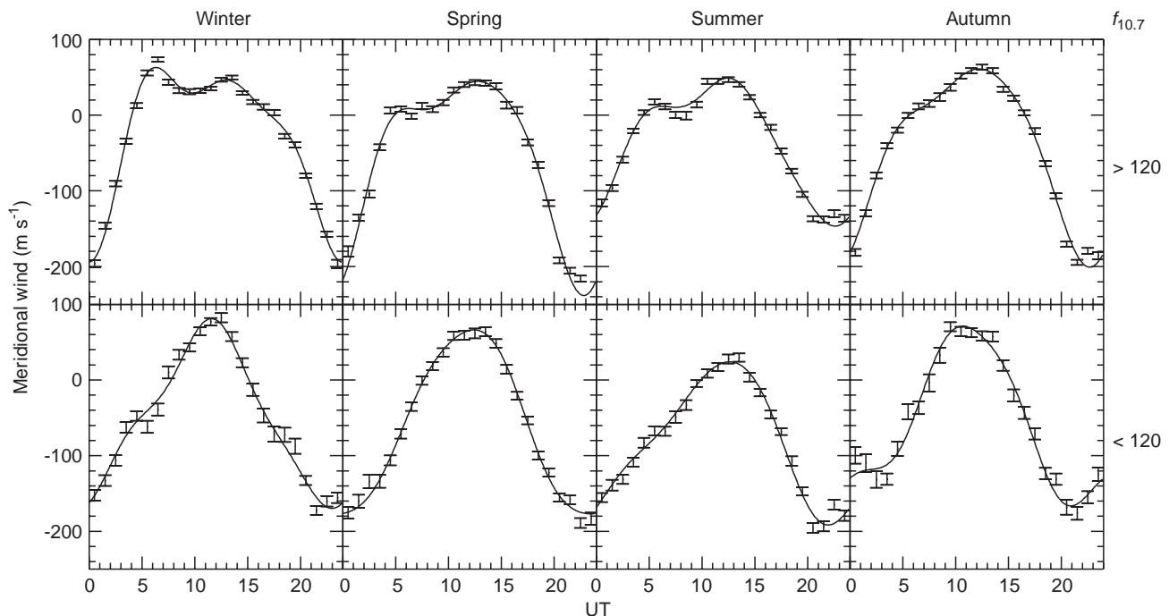
Fig. 4. Mean wind patterns ( points with errorbars ) and the harmonic fit ( solid line ) at 257 km height. Different classes are represented as in Table 2. The first line of boxes corresponds to high solar fluxes, the
