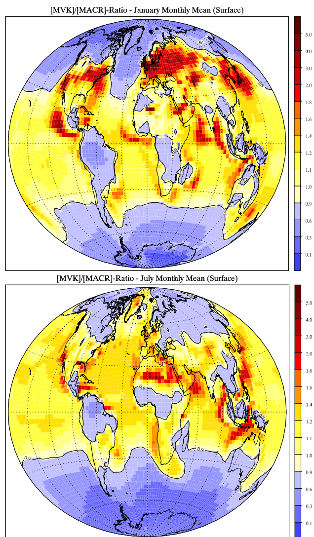
Fig. 19. Ratio of the monthly mean methyl vinyl ketone and methacrolein surface mixing ratios, [\text{MVK}]/[\text{MACR}] , for January and July.
