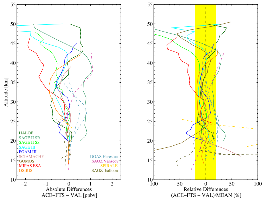
Fig. 38. Summary plot for all the comparisons with ACE-FTS NO 2 . Left panel: Profiles of the mean absolute differences. Right panel: Profiles of the mean relative differences. In both panels, satellite comparisons are indicated by solid lines and other profile comparisons are indicated by dashed lines. Highlighted in yellow are the \pm 20\% relative differences. Note that for SAGE II the results are separated into sunrise and sunset profiles. GOMOS is only present in the right hand panel, because no VMRs are available.
