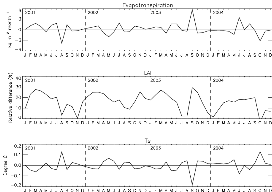
Fig. 3. Impact of the 2050 scenario ([CO 2 ] of 550 ppm) on winter wheat, for four contrasting years (Y1 to Y4, Table 1). From top to bottom: difference in monthly evapotranspiration, relative difference in LAI, monthly average difference in leaf temperature.
