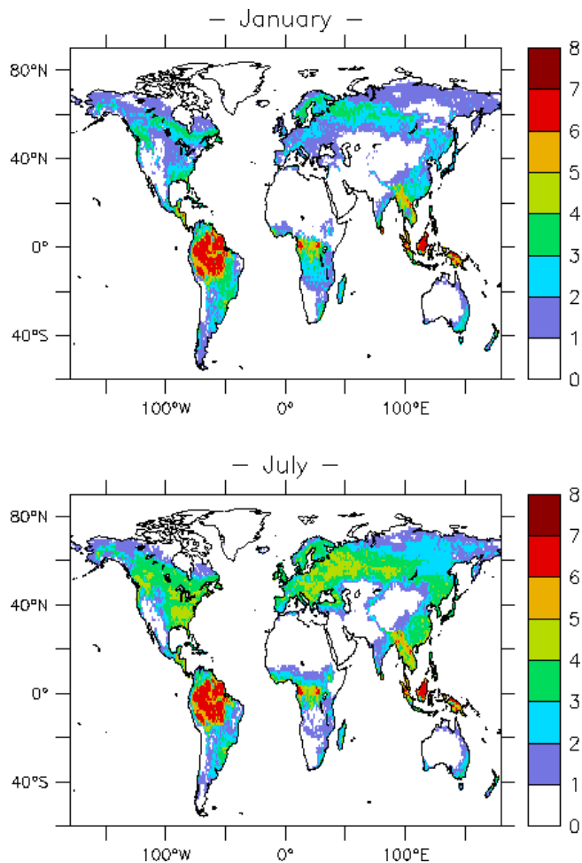
Fig. 2. Monthly mean Leaf Area Index (LAI, \text{m}^2/\text{m}^2 ) calculated by ORCHIDEE for January and July.
