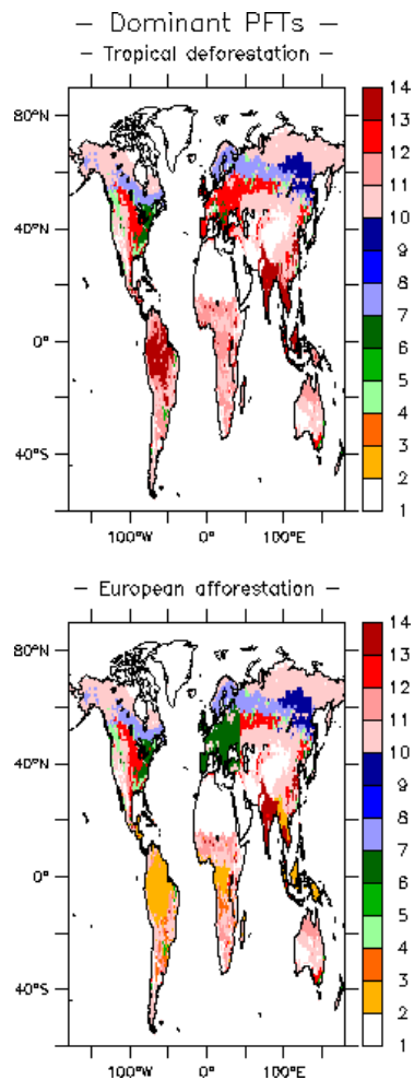
Fig. 7. PFTs distribution considered for the Tropical deforestation (upper panel) and European afforestation (lower panel) scenarios.
