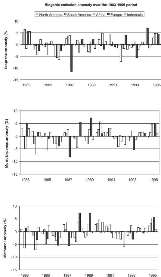
Fig. 6. Variability of annual biogenic emissions anomaly based on 1983–1995 mean emissions calculated for North America, South America, Africa, Europe and Indonesia for isoprene (upper panel), monoterpenes (middle panel) and methanol (lower panel).
