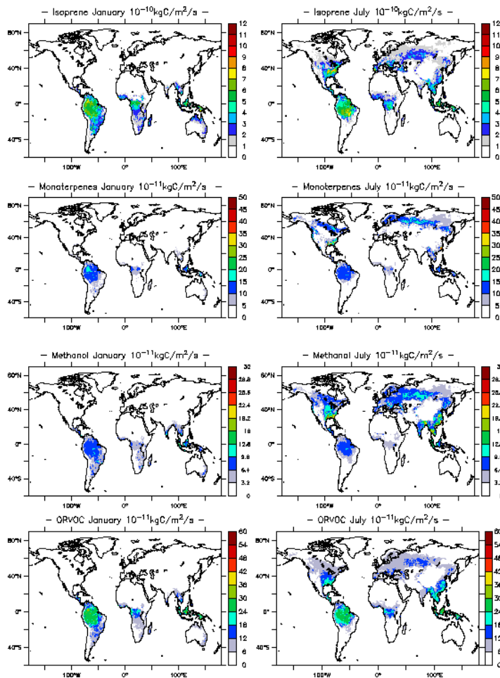
Fig. 3. Global mean biogenic emissions over the 1983–1995 period in \text{kgC/m}^2/\text{s} in January (left column) and July (right column) for isoprene, monoterpenes, methanol and ORVOC.
