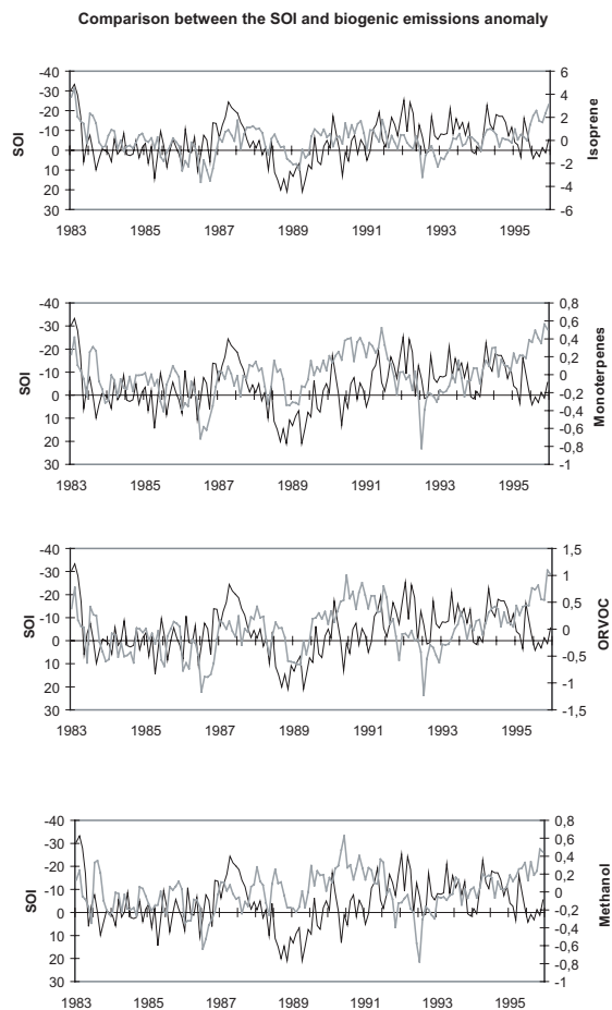
Fig. 4. Comparison between the Southern Oscillation Index SOI (black line) and the simulated anomalies of global monthly biogenic emissions (grey line, TgC/month) for the 1983–1995 period.
