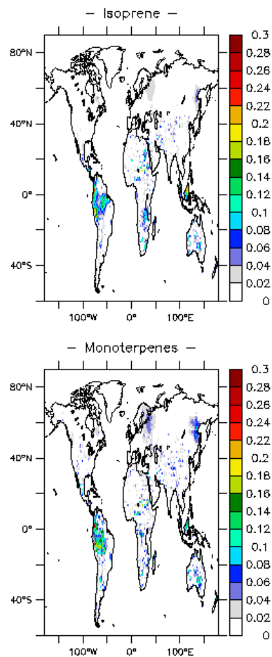
Fig. 5. Square correlation coefficient ( r^2 ) between the Southern Oscillation Index and biogenic emissions for the 1983–1995 period for isoprene (upper panel) and monoterpenes (lower panel).
