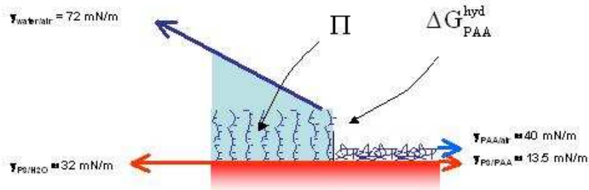
Figure 12: Illustration of the thermodynamic model, which takes into account the interfacial energies \gamma_{PS/H_2O} , \gamma_{H_2O/air} , \gamma_{PS/PAA} , \gamma_{PAA/air} , the enthalpy of hydration of AA monomers \Delta G_{PAA}^{hyd} , and the interfacial pressure inside the brush \Pi .
