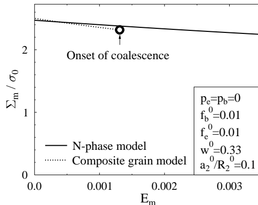
Fig. 7. Onset of void coalescence detected by the composite grain model.
