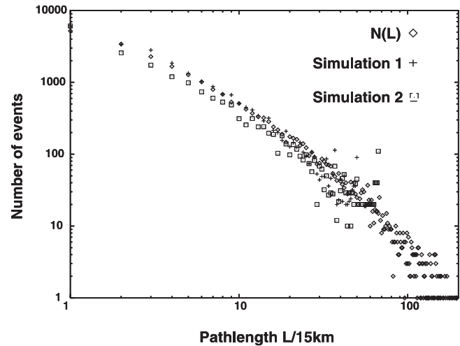
Fig. 5. Frequency distribution of path lengths inside ISSR according to two different numerical simulations using circular ISSRs with diameters distributed according to a generalised gamma-density, compared to the original data, N(L)
