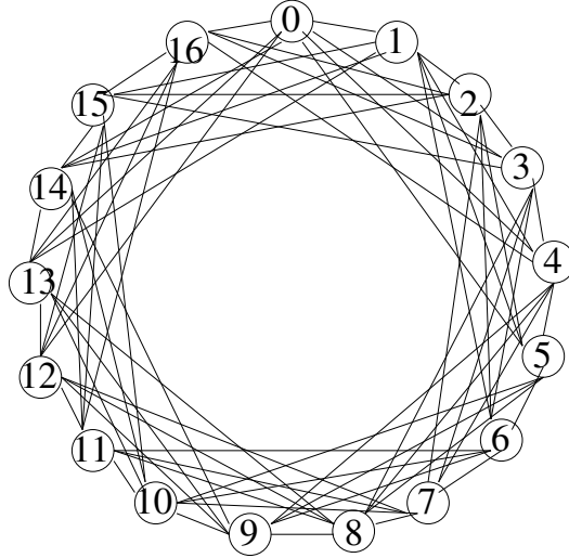
Fig. 1. The circular partitionable graph C[2, 2, 2, 2]
