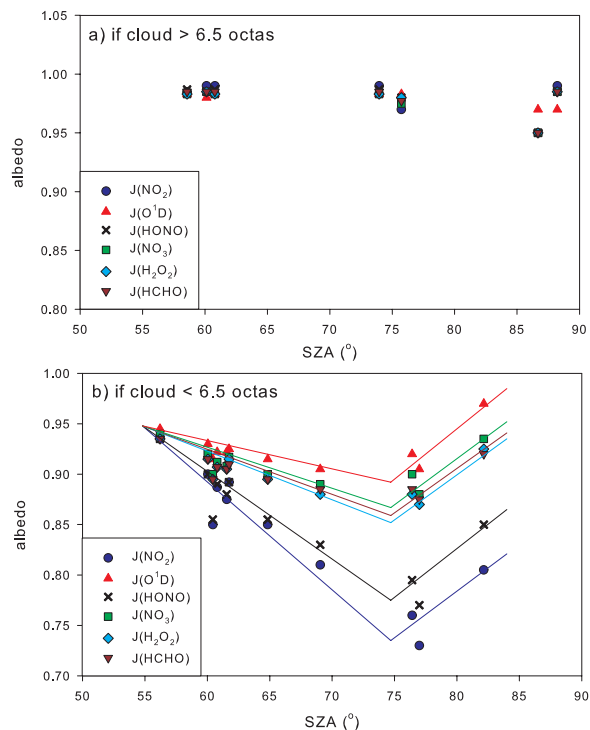
Fig. 13. Hemispheric albedo (i.e. a 2\text{-}\Pi average) derived from j-values for specific molecules. These were calculated from spectra measured by the actinic flux spectrometer at Halley in January and February 2005 (a) in cloudy conditions, and (b) less cloudy conditions, as a function of solar zenith angle (SZA). In the upper plot, albedo is constant with SZA and has a variability of around 0.5%. Pairs of straight lines in the lower plot are fits by hand to the points, to enable models to use albedos in less cloudy conditions within a few percent, interpolated to SZA values, on any day of the year. Albedos in cloudy conditions are about 0.98 irrespective of SZA.
