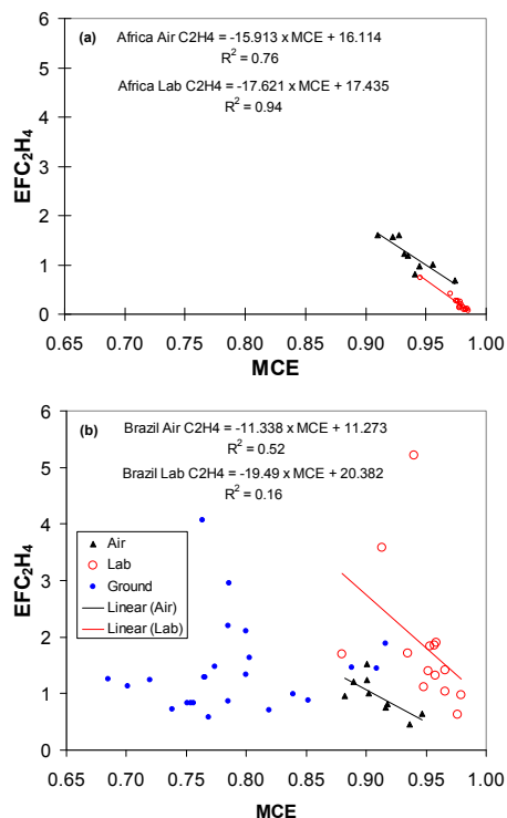
Fig. 4. (a) The relevant range of fire-integrated MCE for savanna fires is about 0.90–0.98. For C 2 H 4 , over this range, the EF from airborne measurements of African savanna fires and the lab EF measured using savanna fuels are in good agreement with each other and highly correlated with MCE. (b) The agreement between the lab and air and the correlation with MCE decreases for tropical forest fire EF. Including the ground-based field data indicates that EFC 2 H 4 may be fuel dependent (lower from woody material than foliage) and/or not uniquely identified with either flaming or smoldering combustion.
