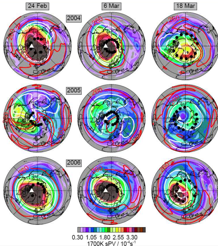
Fig. 1. Maps of scaled Potential Vorticity (sPV, 10^{-4}\text{s}^{-1} ) from GEOS-4 on the 1700 K isentropic surface ( \sim 1.5\text{ hPa} , \sim 50\text{ km} ) on (left to right) 24 February, 6 March and 18 March in (top to bottom) 2004 through 2006. Contours are GEOS-4 temperatures of 240, 250, 260 and 270 K (lower two white, higher two red). Black dots show ACE-FTS observation locations and white triangle shows the location of Eureka. Projection is orthographic, from 0^\circ to 90^\circ\text{ N} , with 0^\circ longitude at the bottom and 90^\circ\text{ E} to the right.
