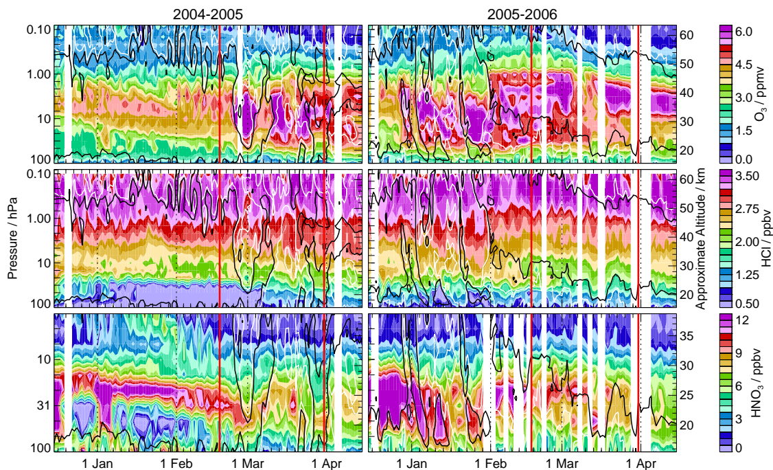
Fig. 15. As in Fig. 14, but for (top to bottom) MLS v1.5 O 3 , HCl and HNO 3 . Vertical range for O 3 and HCl is into the lower mesosphere; vertical range for HNO 3 is into the upper stratosphere.
