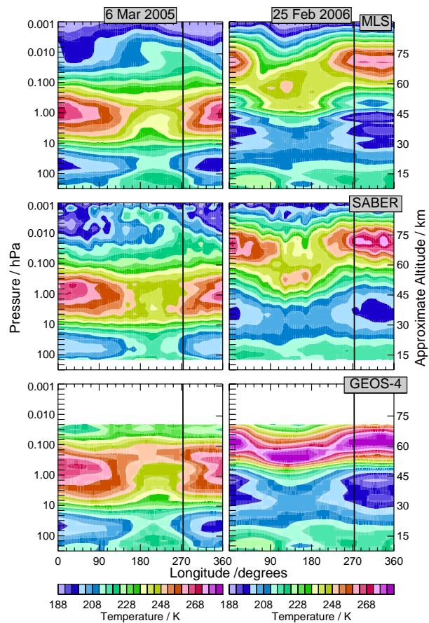
Fig. 11. As in Fig. 10, but for 6 March 2005 and 25 February 2006, and showing (top to bottom) MLS v2.2, SABER and GEOS-4 temperatures.
