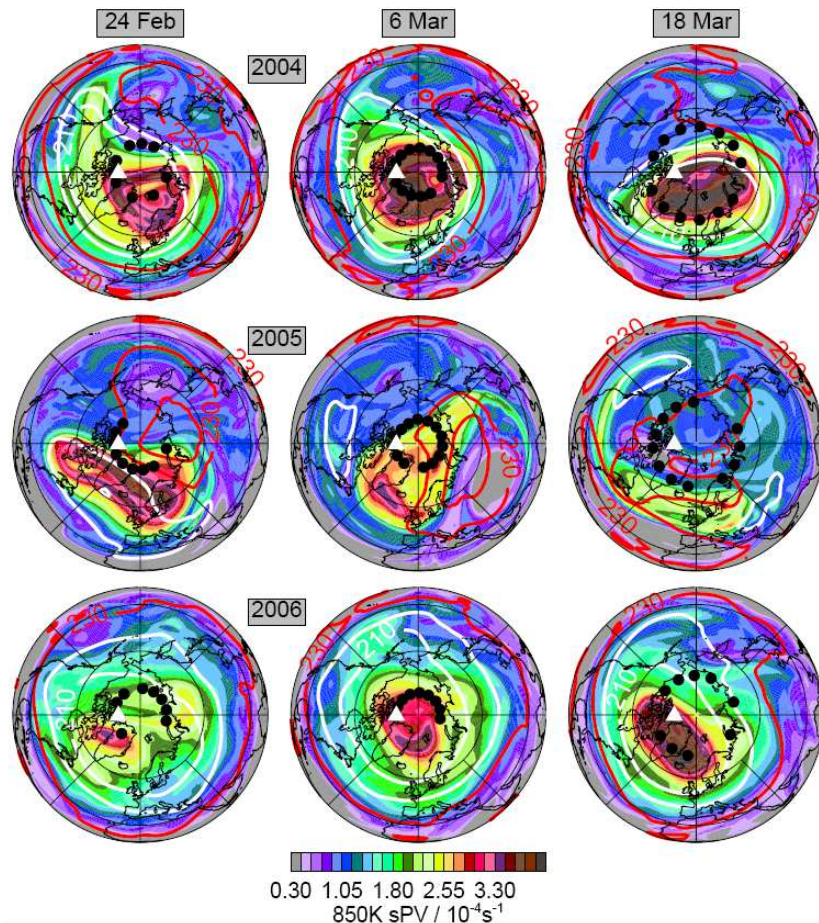
Fig. 2. As in Fig. 1, but at 850 K ( \sim 10 hPa, \sim 30 km), and with temperature overlays of 210, 220, 230 and 240 K (lower two white, higher two red).
