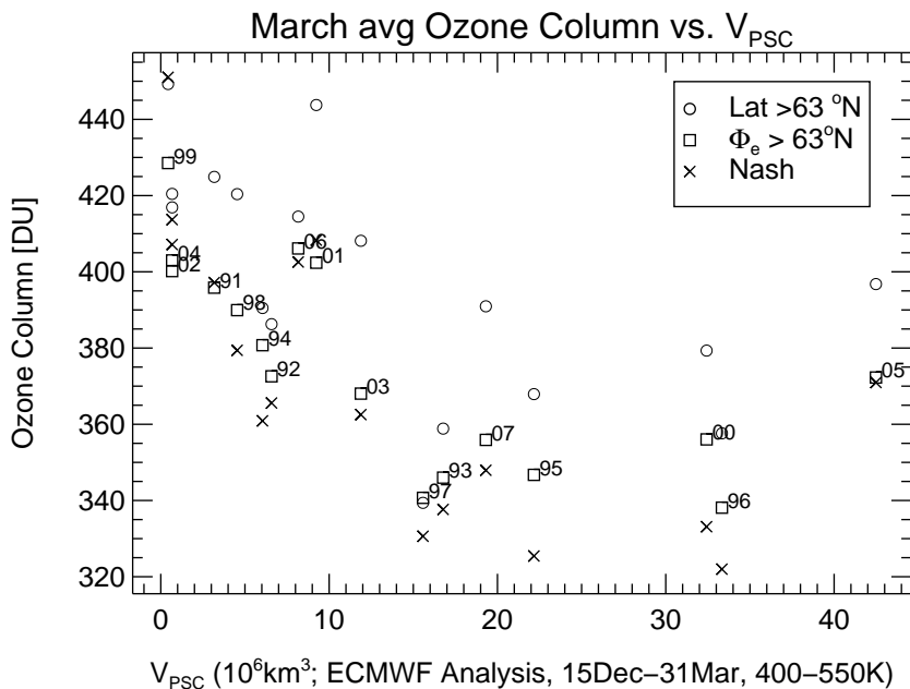
Fig. 10. The relation between V_{PSC} and the total column ozone in March averaged over the Arctic polar region. Circles show averages poleward of 63°N, squares averages poleward of 63°N equivalent latitude, and crosses averages poleward of the vortex edge defined by the maximum gradient in potential vorticity.
