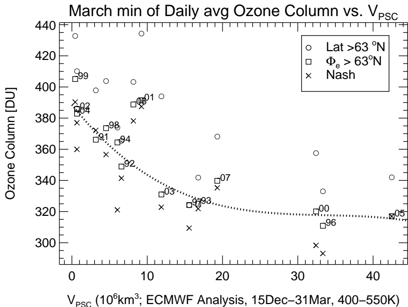
Fig. 11. The relation between V_{\text{PSC}} and the minimum of March daily average polar column ozone (symbols as in Fig. 10). The dotted line shows an empirical fit through the minimum ozone values for averages poleward of an equivalent latitude of 63^\circ\text{N} with the exception of the years 1999, 2001, and 2006 for which the final warming occurred before March. Not shown (and excluded from the fit) is the year 1995 because of poor data quality; only 3% of the data points poleward of 63^\circ equivalent latitude are valid. The polynomial describing the fit is given by M = 388.6 - 6.10 \cdot V + 0.178 \cdot V^2 - 0.00176 \cdot V^3 , where V is V_{\text{PSC}} in 10^6 \text{ km}^3 and M is the minimum of March daily average polar column ozone in Dobson units (this relation being valid for V_{\text{PSC}} < 42.5 ).
