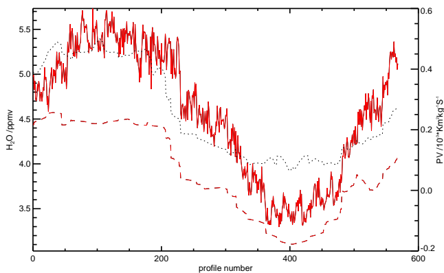
Fig. 11. ECMWF water vapour (red, dashed), PV (black, dotted) and AMSOS water vapour (red, solid) on the 850 K isentrope at mission 5 locations.
