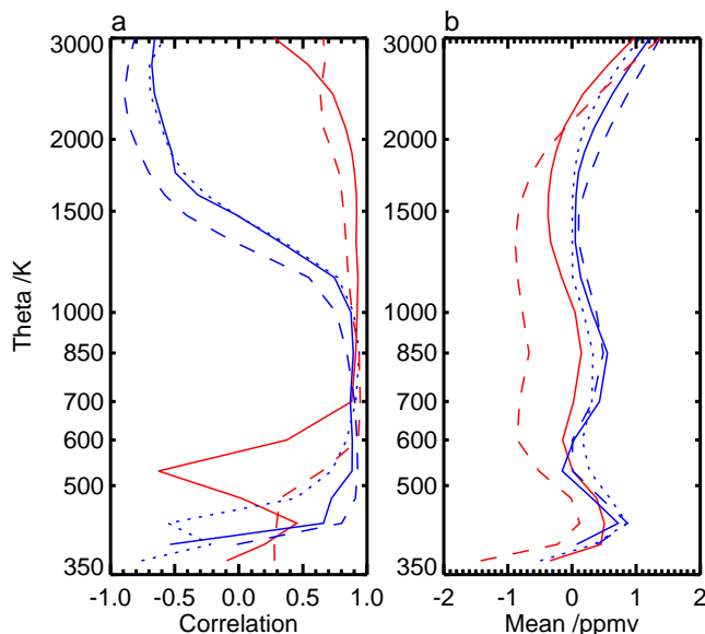
Fig. 6. (a) Pearson correlation coefficient between ECMWF and AMSOS humidities, and (b) Mean of ECMWF – AMSOS humidity, evaluated on isentropic levels and using all available retrievals from missions 1 (1998, solid red), 2 (1999, solid blue), 3 (2000, dashed blue), 4 (2001, dotted blue) and 5 (2002, dashed red). Red denotes a summer mission and blue a winter mission.
