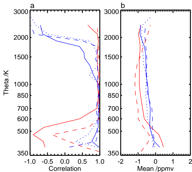
Fig. 7. (a) Pearson correlation coefficient between ECMWF humidities and UARS climatology humidities, and (b) Mean of ECMWF – UARS climatology. Other details as for Fig. 6.
