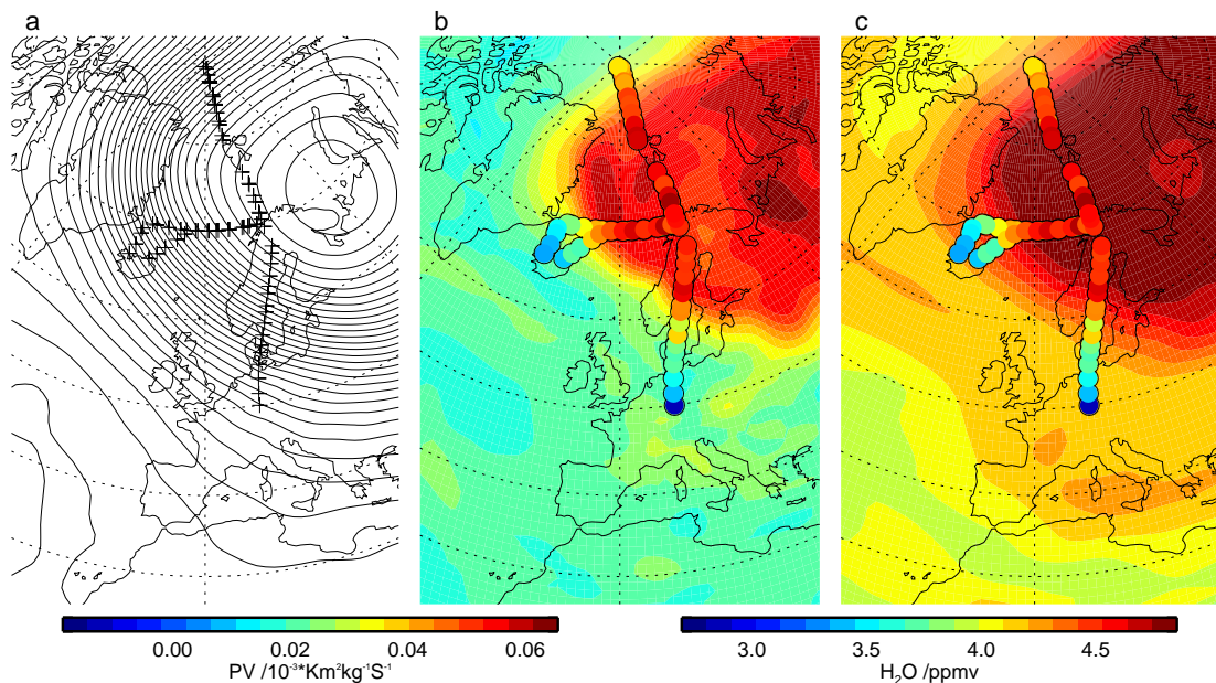
Fig. 10. ECMWF analyses for 12:00:00 UT 9 March 2000: (a) Geopotential height on a 50 hPa surface with AMSOS observation points; (b) Potential vorticity on the 475 K isentrope with AMSOS water vapour overlaid; (c) Water vapour mixing ratio on the 475 K isentrope with AMSOS water vapour overlaid. AMSOS observations from 8 March 2000 to 10 March 2000 are shown.
