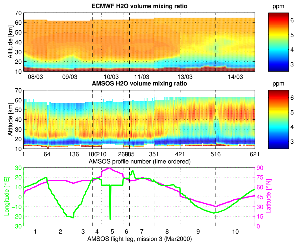
Fig. 3. Overview of the complete AMSOS Mission 3 (8–14 March 2000). The top plot shows ECMWF ERA-40 humidity profiles that correspond to the measured AMSOS profiles in the centre plot. The bottom plot shows the position of the measurements. The AMSOS profiles are ordered by time and numbered. Measurements from different days are separated by vertical dashed lines, while dotted lines separate different flight legs.
