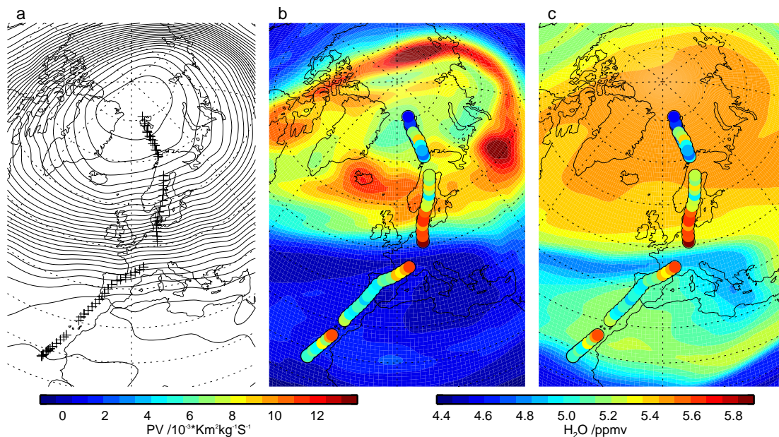
Fig. 9. ECMWF analyses for 12:00:00 UT on 6 February 1999: (a) Geopotential height on a 2 hPa surface with AMSOS observation points; (b) Potential vorticity on the 1475 K isentropes with AMSOS water vapour overlaid; (c) Water vapour mixing ratio on the 1475 K isentropes with AMSOS water vapour overlaid.
