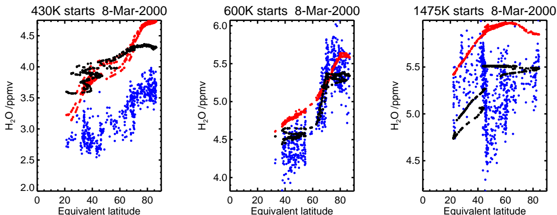
Fig. 5. AMSOS retrievals in March 2000 (blue), and at AMSOS locations the UARS climatology (red) and ECMWF analyses (black), against PV equivalent latitude on isentropic surfaces at (a) 430 K, (b) 600 K and (c) 1475 K.
