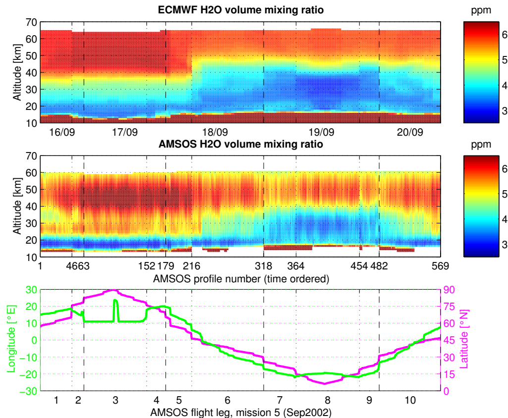
Fig. 4. Similar to Fig. 3 but for AMSOS Mission 5 (16–20 September 2002). The ECMWF humidity profiles are from the operational data set because ERA-40 ended in August 2002.
