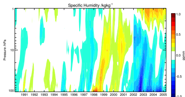
Fig. 1. Time series of deseasonalised humidity anomalies from the ECMWF analyses, averaged over the region 20° S to 20° N. ERA-40 analyses are presented up until December 2001; operational analyses thereafter.
