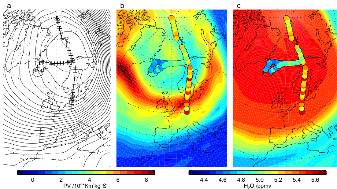
Fig. 8. ECMWF analyses for 12:00:00 UT on 9 March 2000: (a) Geopotential height on a 2 hPa surface with AMSOS observation points; (b) Potential vorticity on the 1475 K isentropes with AMSOS water vapour overlaid; (c) Water vapour mixing ratio on the 1475 K isentropes with AMSOS water vapour overlaid. AMSOS observations from 8 March 2000 to 10 March 2000 are shown.
