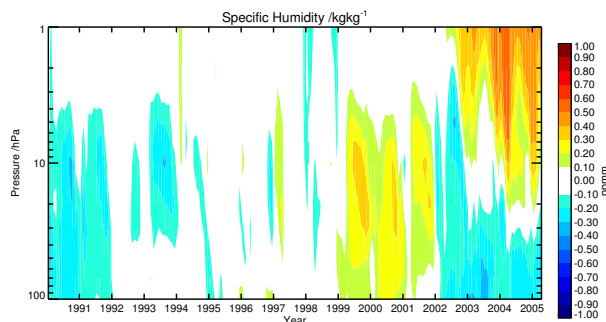
Fig. 2. Time series of deseasonalised humidity anomalies from the ECMWF analyses, averaged over the region 70°N to 90°N. ERA-40 analyses are presented up until December 2001; operational analyses thereafter.
