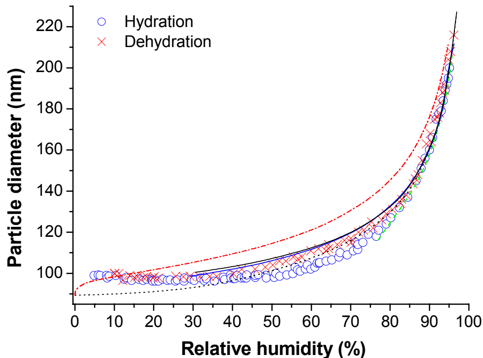
Fig. 8. Mobility equivalent diameters of deliquesced \text{NH}_4\text{NO}_3 particles with D_{b,i} = 99 nm observed upon hydration (H-TDMA mode 1) and dehydration (H-TDMA mode 2) compared to Köhler theory calculations with D_{m,\text{NH}_4\text{NO}_3} = D_{b,h\&d,\text{min}} = 89 nm and different models: VA with \Phi_{\text{NH}_4\text{NO}_3} = 1 , red dash-dotted; VA with \Phi_{\text{NH}_4\text{NO}_3} from Brechtel and Kreidenweis (2000), green dashed; VA with a_w from Clegg et al. (1998), black dotted; VA with \Phi_{\text{NH}_4\text{NO}_3} from Brechtel and Kreidenweis (2000), green dashed; FP with a_w from Clegg et al. (1998) and \rho from Tang (1996), black solid; FP with a_w and \rho from Tang (1996), blue solid.
