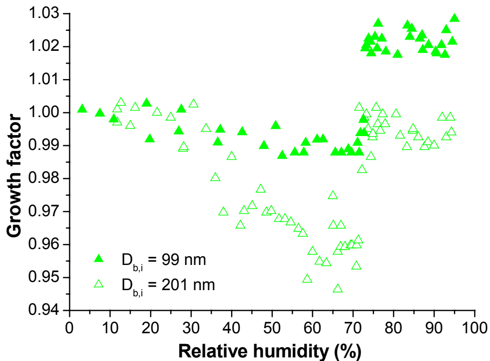
Fig. 5. Mobility equivalent growth factors of NaCl particles with D_{b,i} = 99 \text{ nm} and D_{b,i} = 201 \text{ nm} observed upon hydration & dehydration (H-TDMA mode 3, RH_2 ).
