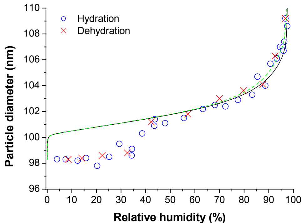
Fig. 11. Mobility equivalent diameters of pure BSA particles with D_{b,i} = 98 nm observed upon hydration (H-TDMA mode 1) and dehydration (H-TDMA mode 2) compared to Köhler theory calculations with D_{m,BSA} = D_{b,i} = 98 nm and the VA model based on \Phi_{BSA} from osmotic pressure parameterisation: Kelvin term with \sigma = \sigma_w , black solid; Kelvin term with \sigma = 0 , dashed green.
