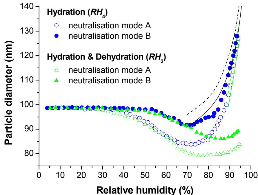
Fig. 16. Mobility equivalent diameters observed in H-TDMA modes 1 and 3 and neutralisation modes A and B for mixed \text{NH}_4\text{NO}_3 -BSA particles with D_{b,1} = 99 nm and 50% BSA dry mass fraction compared to Köhler theory calculations using the SS-VA model with different parameterisations and dry solute mass equivalent diameters: a_w from Clegg et al. (1998), black; \Phi_{\text{NH}_4\text{NO}_3} from Brechtel and Kreidenweis (2000), green; D_{m,s} = D_{b,hy,min} , dashed; D_{m,s} = D_{b,h\&d,min} , solid.
