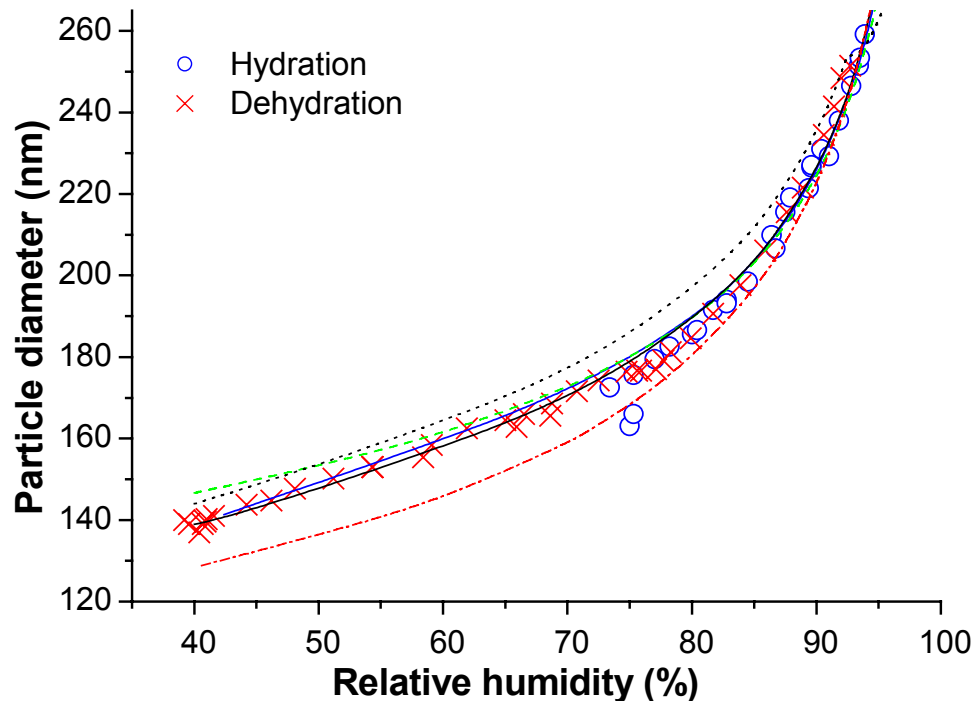
Fig. 7. Mobility equivalent diameters of deliquesced NaCl particles with D_{b,i} = 99 nm observed upon hydration (H-TDMA mode 1) and dehydration (H-TDMA mode 2) compared to Köhler theory calculations with D_{m,NaCl} = D_{hy,min,hicorr} = 95 nm (except black dotted line with D_{m,NaCl} = D_{b,i} = 99 nm) and different models: VA with \Phi_{NaCl} = 1 , red dash-dotted; VA with \Phi_{NaCl} from Brechtel and Kreidenweis (2000), green dashed; FP with \Phi_{NaCl} from Mokbel et al. (1997) and \rho from Tang (1996), black solid and dotted; FP with a_w and \rho from Tang (1996), blue solid.
