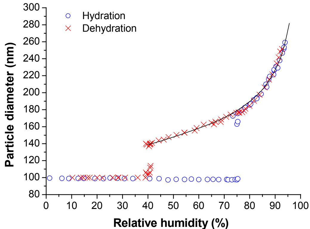
Fig. 3. Mobility equivalent diameters of NaCl particles with D_{b,i} = 99 nm observed upon hydration (H-TDMA mode 1) and dehydration (H-TDMA mode 2) compared to Köhler theory calculations with the FP model based on \Phi_{\text{NaCl}} from Mokbel (1997), \rho from Tang (1996), and D_{m,s} = 95 nm.
