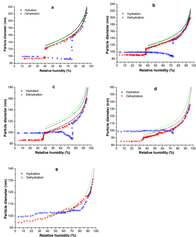
Fig. 13. Mobility equivalent diameters observed upon hydration (H-TDMA mode 1) and dehydration (H-TDMA mode 2) of mixed NaCl-BSA particles with D_{b,i} = 99 nm and BSA dry mass fractions of 10% (a), 25% (b), 50% (c), 75% (d), and 90% (e) compared to Köhler theory calculations with different VA models ( \Phi_{\text{NaCl}} from Mokbel et al., 1997; \Phi_{\text{BSA}} from osmotic pressure parameterisation) and dry solute mass equivalent diameters: AS-VA, green; SS-VA, black; D_{m,s} = D_{b,hy,min} , dotted (a, b); D_{m,s} = D_{b,de,min} , dashed (c, d, e); D_{m,s} = D_{m,hy,min} , solid (a, b); D_{m,s} = D_{b,h\&d,min} , solid (c).
