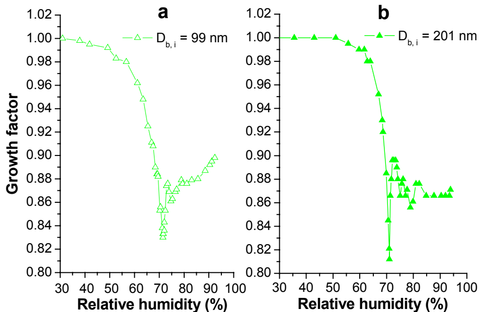
Fig. 15. Mobility equivalent growth factors of NaCl-BSA particles with 50 % BSA dry mass fraction, D_{b,i} = 99 nm (a) and D_{b,i} = 201 nm (b) observed upon hydration & dehydration (H-TDMA mode 3, RH_2 ).
