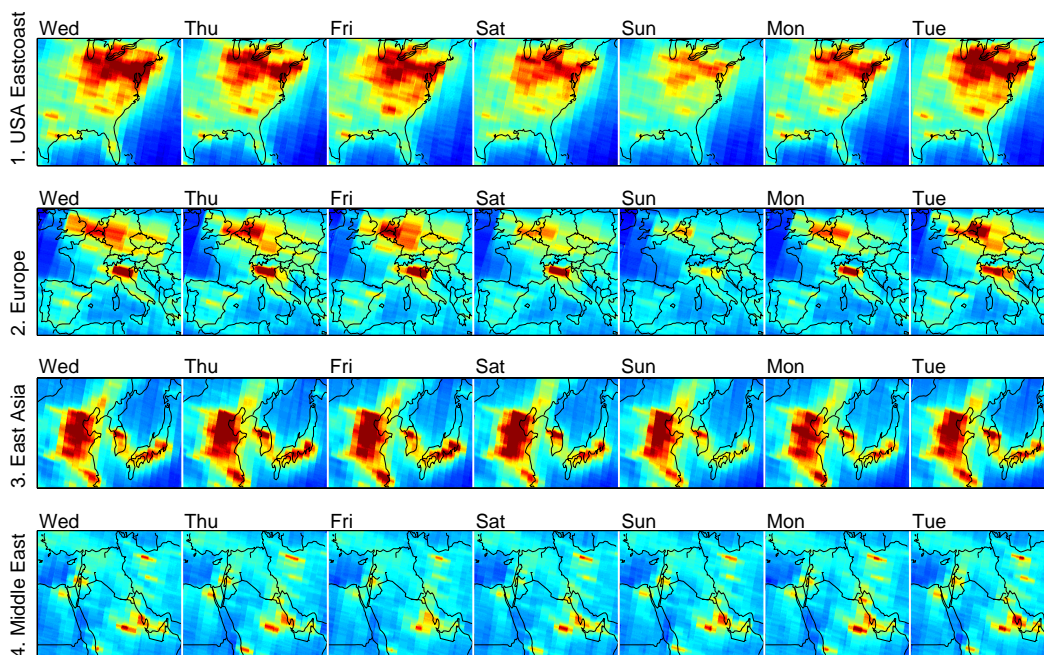
Fig. 2. Mean tropospheric NO 2 VCD (1996–2001) for the regions of interest, as marked in Fig. 1, for the different days of the week separately. Colour scale and unit are the same as in Fig. 1.
