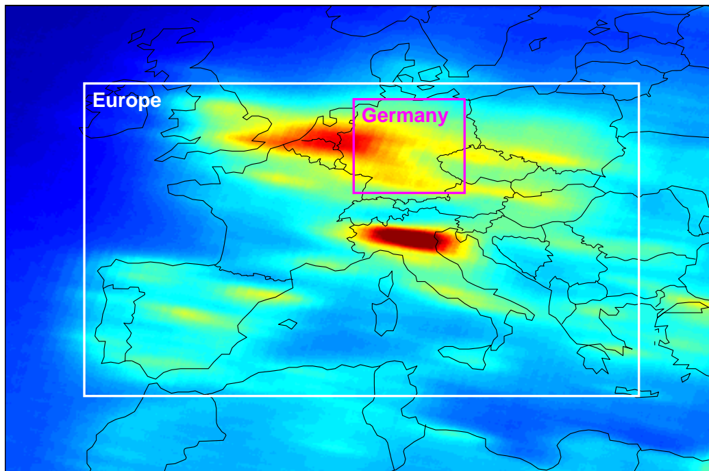
Fig. 4. Zoom of Fig. 1 on West Europe. For the lifetime estimation of tropospheric NO 2 in Germany, the considered area is marked (7°–14° E and 48°–54° N).
