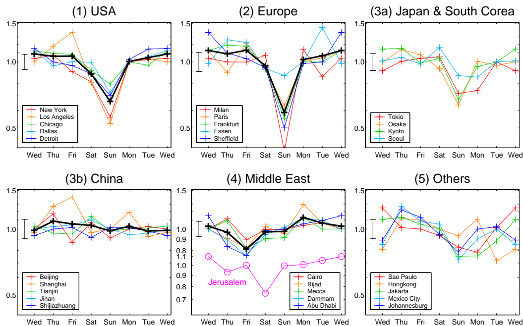
Fig. 3. Weekly cycle of tropospheric NO 2 VCD for the considered locations (as marked in Fig. 1). The values are normalized with respect to the median weekly value (relative units). Black lines are averaged curves. The error bar to the left of every plot indicates the maximum error (standard error of the mean) of all data points.
