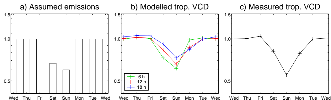
Fig. 5. Weekly cycle of NO 2 (modelled and measured) for Germany (as shown in Fig. 4). All plots are normalized with respect to the median weekly value (relative units). (a) Assumed weekly cycle of NO x emissions (Adopted from Wickert, 2001). (b) Modelled tropospheric VCD at ERS-2 overflight time for different lifetimes of NO 2 . (c) Mean tropospheric VCD of NO 2 measured with GOME.
