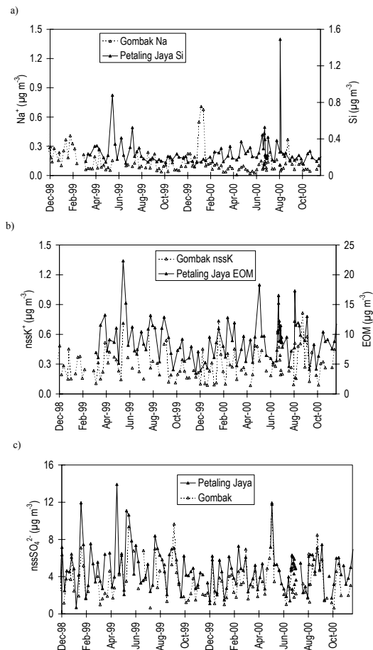
Fig. 6. Time series of (a) \text{Na}^+ at Gombak and Si at Petaling Jaya, (b) nssK ^+ at Gombak and EOM at Petaling Jaya and (c) nssSO _4^{2-} at both sites measured in 24-h PM _2.5 aerosol samples.
