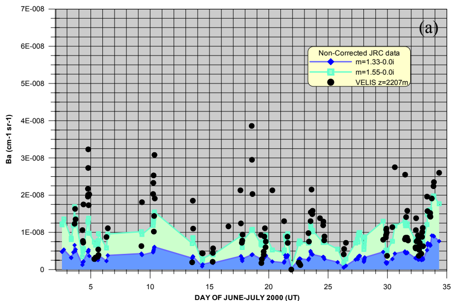
Fig. 2. Lidar observed (black dots) and size distribution-derived backscatter coefficients for two values of the refractive index: 1) m = 1.33-0.0i (diamonds), 2) m = 1.55-0.0i (open squares). Results employing original DMA “dry” size distributions are presented in (a), while (b) considers particles RH -dependent growth.
