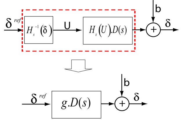
Fig. 7. The scheme of the feedforward control.
