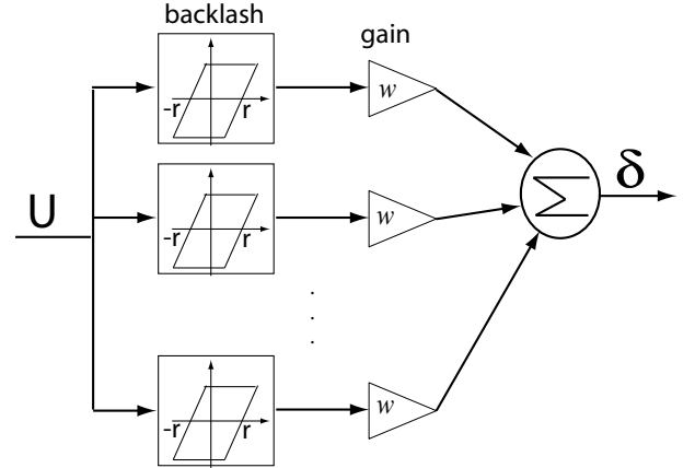
Fig. 8. The PI static hysteresis model.
