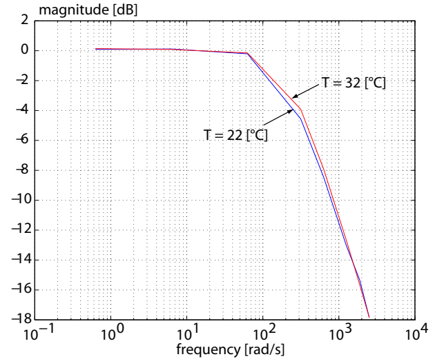
Fig. 14. Frequency response.
