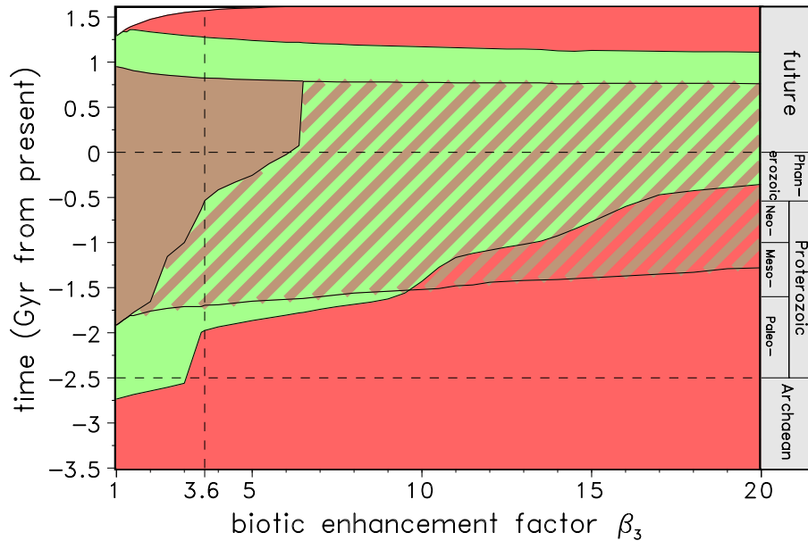
Fig. 2. Stability diagram for the three types of biosphere as a function of the biotic enhancement factor, \beta_3 . In the red area only prokaryotic life exists while in the green area eucaryotic and prokaryotic life coexist. In the brown area complex multicellular life appears additionally. The dashed area indicates the time interval in which a perturbation may trigger the first emergence or extinction of complex multicellular life prematurely.
