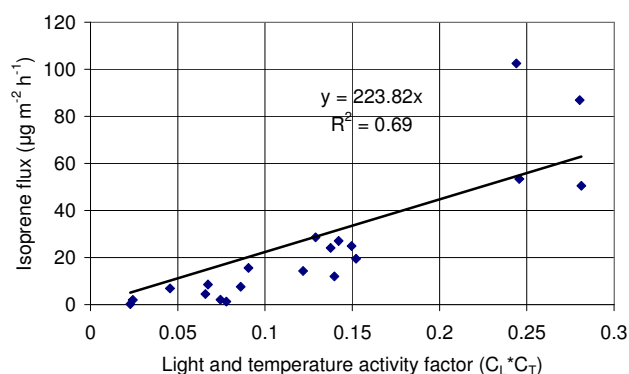
Fig. 1. Light and temperature dependence of measured isoprene emission rates on Siikanen fen.
