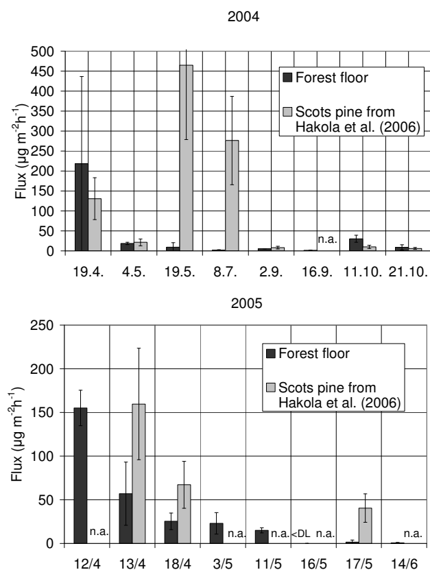
Fig. 3. Sum of the measured emission rates of the terpenes from the forest floor and Scots pine (for biomass density 300\text{ g m}^{-2} ) at Hyytiälä in 2004 and 2005. The Scots pine results are from the study of Hakola et al. (2006). Data for Scots pine emissions on 16th of September 2004 were missing and in 2005 data were only available for 13 and 18 April and for 17 May. (Bars=daily average and error bars=standard deviations between the samples)
