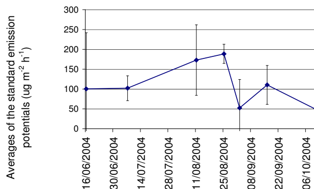
Fig. 2. Standard ( 30^\circ\text{C} and 1000 \mu\text{mol m}^{-2} \text{h}^{-1} ) emission potentials of the isoprene on the Siikanen fen in 2004. (Dots=daily averages and Error bars= 2 \times Standard error of mean).
