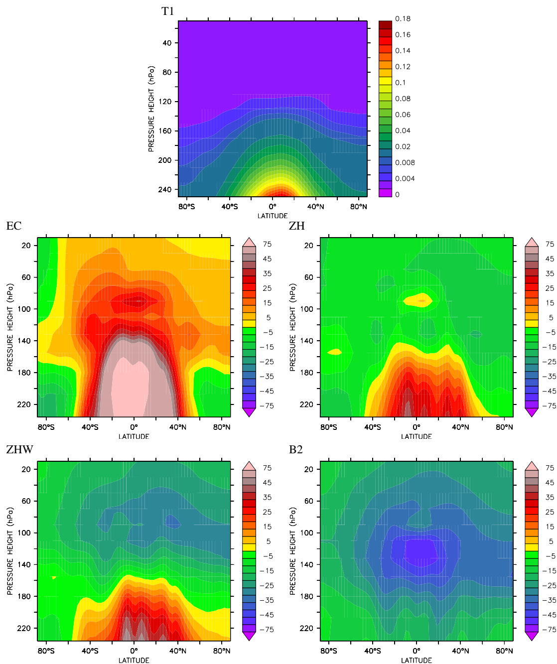
Fig. 5. Zonal average specific humidity (6 year average) above 250 hPa. The upper panel shows the zonal distribution from the T1 reference simulation in g_{\text{water}}/kg_{\text{air}} . The other panels depict the relative differences in % to this reference.
