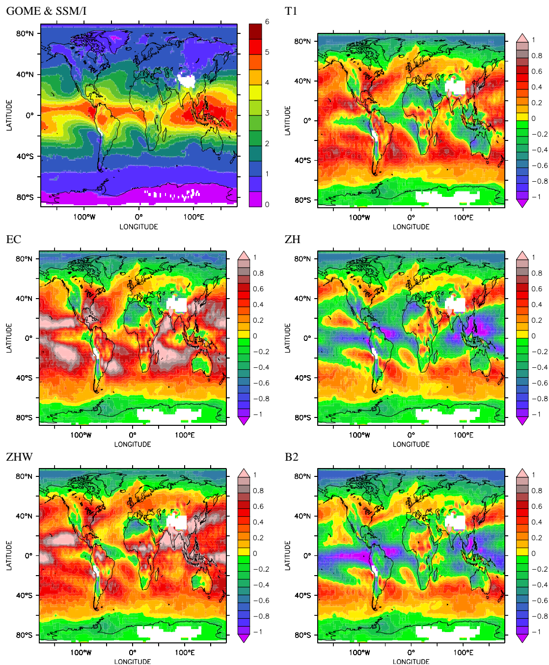
Fig. 4. Horizontal distribution of the annual average (5 years) IWVC in cm. The upper left panel shows the observed values, while the others depict the differences between the individual simulations and the observations (model minus observations) in cm. White areas are regions for which no observations are available.
