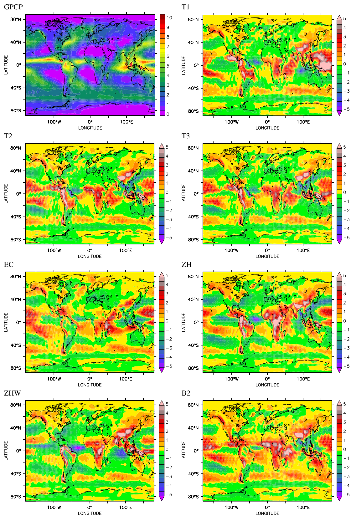
Fig. 2. Observed and simulated horizontal distribution of precipitation in mm/day (6 year average). The upper left panel shows the GPCP (observational data), the other panels the difference between the individual simulations and the observations (model minus observations).
