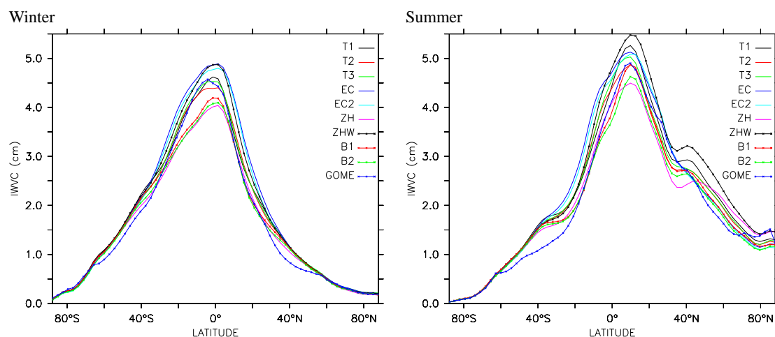
Fig. 3. Zonal average integrated water vapour column in cm for boreal winter (DJF) and summer (JJA) (5 year average).
