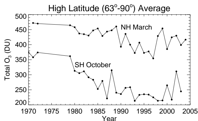
Fig. 1. Time series of average total O 3 from TOMS (version 7) measurements at high latitudes in March and October. Plot is updated from Newman et al. (1997). Data for 1971–1972 are from Nimbus 4 BUV, 1979–1993 from Nimbus 7 TOMS, 1994 from Meteor-3, 1995–1996 from NOAA 9 SBUV/2, 1997 from ADEOS, and data after 1997 from Earth Probe TOMS.
