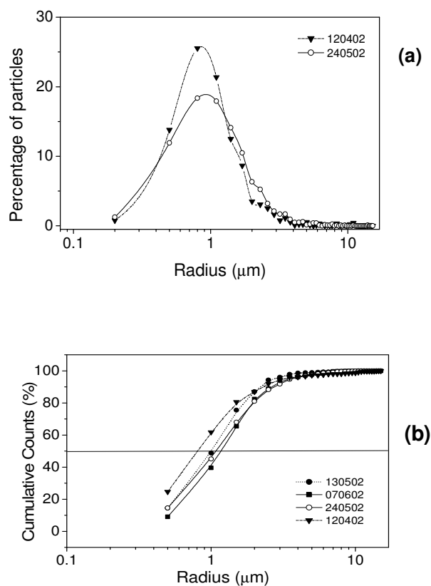
Fig. 6. (a) Typical size distribution of aerosol particles collected during the dust storm of 12 April and 24 May. 913 and 1182 particles have been analyzed on the dust sample of 12 April and 24 May, respectively. (b) Cumulative grain-size curves of the samples collected in the different dust storm events.
