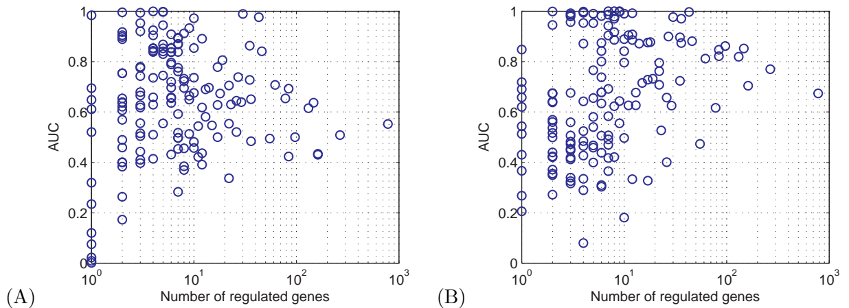
Figure 3: AUC per TF as a function of the number of regulated genes. (A) CLR and, (B) SIRENE
