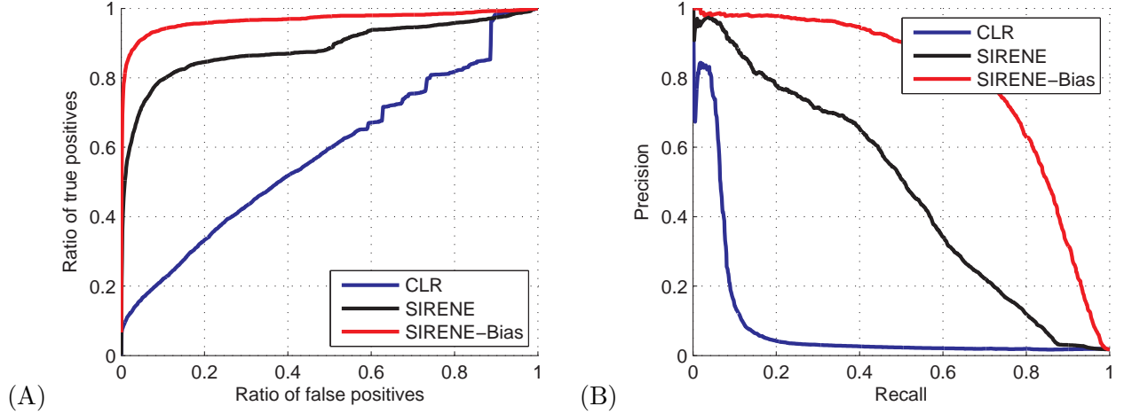
Figure 2: Comparison of performance between CLR and SIRENE. (A) ROC curves, and (B) precision/recall curves. The SIRENE curve corresponds to the SIRENE algorithm evaluated by 3-fold cross-validation, when genes within an operon are never split between the training and the test set. The SIRENE-bias curve is the same algorithm evaluated by classical 3-fold cross-validation, where genes are randomly assigned to training and test sets.
