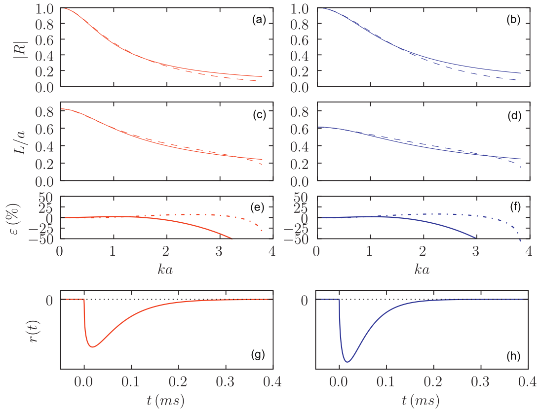
Figure 2: Comparison in frequency domain of the references (dashed lines) and model (\nu, \alpha) of Eqs. (12) through (15) (in solid lines) for the unflanged (left column) and infinitely flanged (right column) cases: modulus |\mathcal{R}(ka)| of the reflection coefficient (first row, approximation error in solid lines in third row), dimensionless length correction L/a (second row, approximation error in dash-dotted lines in third row). An example of the reflection function is given in the last row ( a = 7\text{mm} ).
