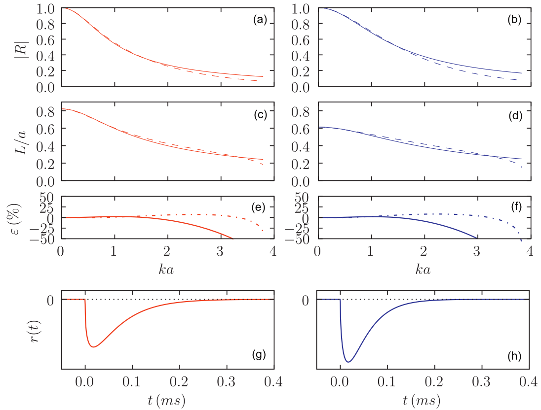
Figure 2: Comparison in frequency domain of the references (dashed lines) and model (\nu, \alpha) of Eqs. (12) through (15) (in solid lines) for the unflanged (left column) and infinitely flanged (right column) cases: modulus |\mathcal{R}(ka)| of the reflection coefficient (first row, approximation error in solid lines in third row), dimensionless length correction L/a (second row, approximation error in dash-dotted lines in third row). An example of the reflection function is given in the last row ( a = 7\text{mm} ).
