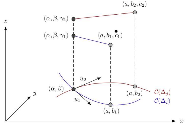
Figure 3: Lifting of an apparent singularity.
