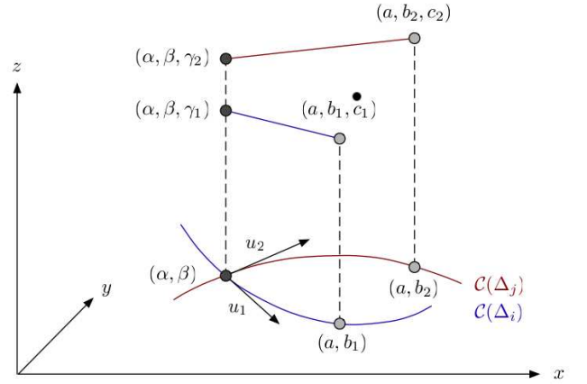
Figure 4: Connection above an apparent singularity.
