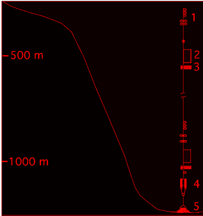
Figure 2. The experimental strategy chosen by the Centre de Formation et de Recherche sur l'Environnement Marin (CEFREM) to study the transfer of the particulate matter from the shelf to the slope on a long time scale. A mooring line is composed by glassed buoys (1), PPS 3 sediment traps located at 500 m (2) and 1,000 m depth (4), Aanderra current-meters RCM with thermistor (3: 500 m depth, 5: 1,000 m depth), an acoustic release system (6), and weight (7) to maintain it since the bottom of the sea. Two mooring lines have been placed in the Gulf of Lion's continental margin. The scientists of the CEFREM conceived the experimental strategy. The technical staff of the CEFREM carried out the samples collection and their treatment.
