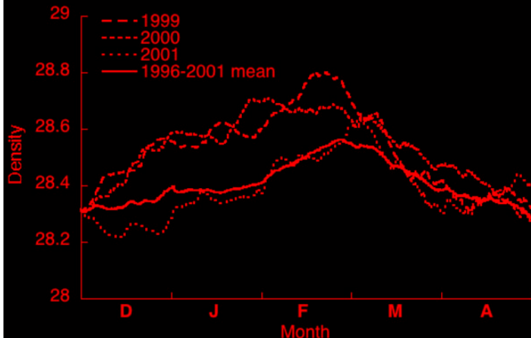
Figure 5. The time evolution of the simulated shelf integrated density for the simulated winter periods. (a) 1996, 1997, 1998 and the 1996-2001 mean, (b) 1999, 2000, 2001 and the 1996-2001 mean.
