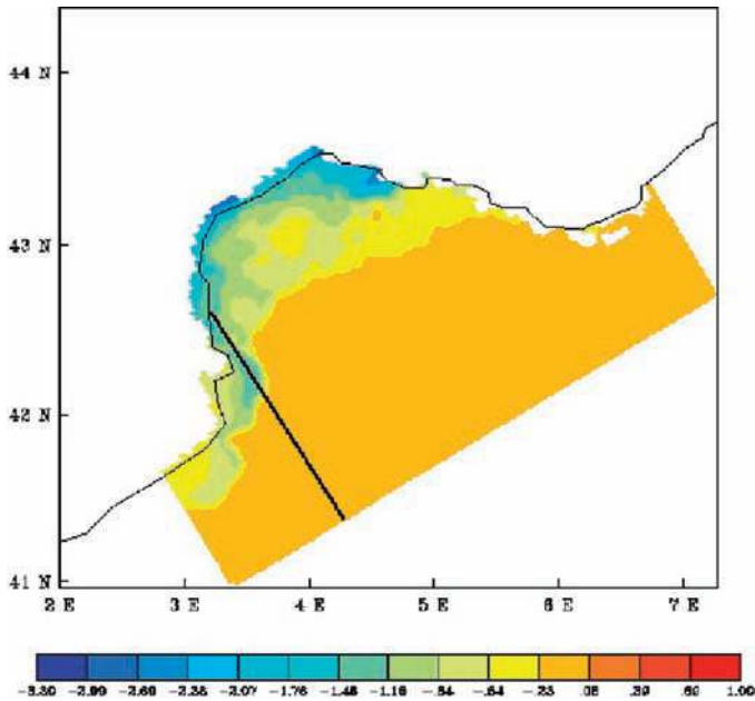
Figure 11. The monthly mean water temperature anomaly in the Gulf of Lion for the 1996 to 2001 winters. This 1996-2001 5 month-period mean water temperature anomaly is shown for the deeper sigma-level of the Symphonie model. The black line represents the section considered to explore the interannual variability of the spread of shelf dense waters at depth. In this figure, the coastline, traced by the visualization tool, is approximated for the GoL, and it does not match perfectly the bathymetry of Symphonie.
