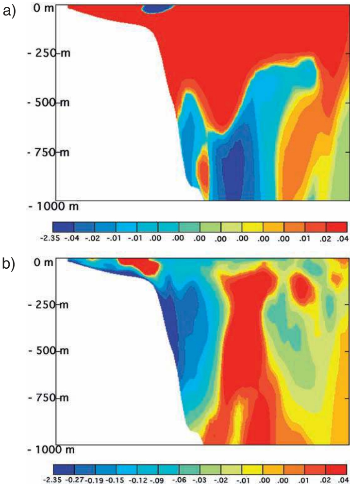
Figure 12. The monthly temperature anomaly section near the Lacaze-Duthiers canyon in (a) March 1997 and (b) March 1999.
