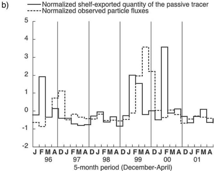
Figure 7. The comparisons of interannual variability of the normalized shelf-exported quantities of the passive tracer and the normalized particulate matter measurements in the Lacaze-Duthiers canyon at 500 meter depth (a) and at 1 000 meter depth (b).
