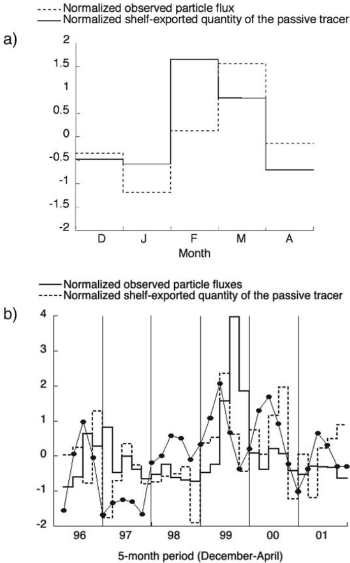
Figure 4. Comparison between normalized observed fluxes and integrated passive tracer over the shelf at different time scales. The mean seasonal cycle (a), and the 5-month interannual variability (b) are shown. The black dotted line represents the month average of the normalized shelf integrated density.
