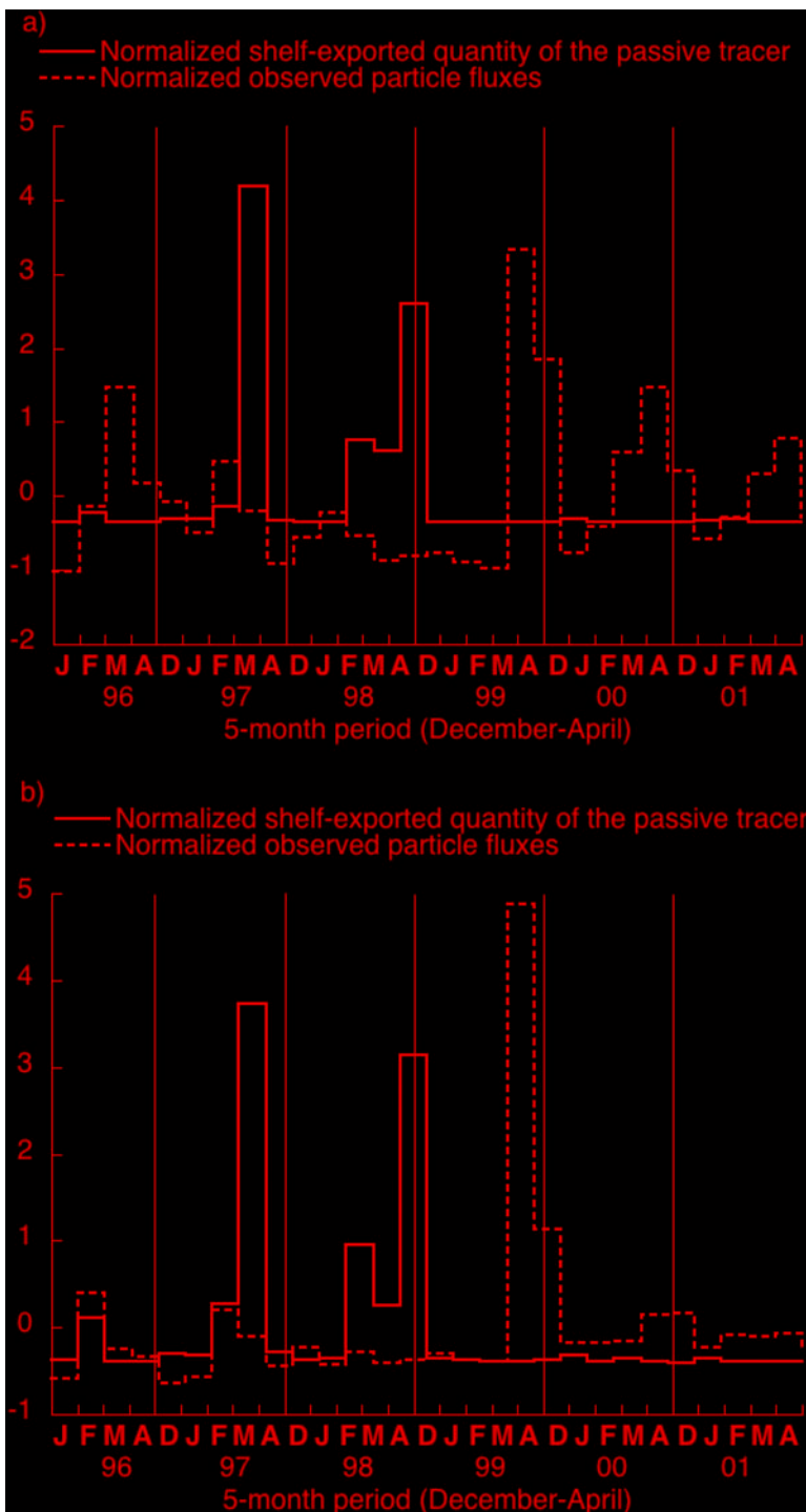
Figure 6. The comparisons of interannual variability of the normalized shelf-exported quantities of the passive tracer and the normalized particulate matter measurements in the Planier Canyon at 500 meter depth (a) and at 1 000 meter depth (b).
