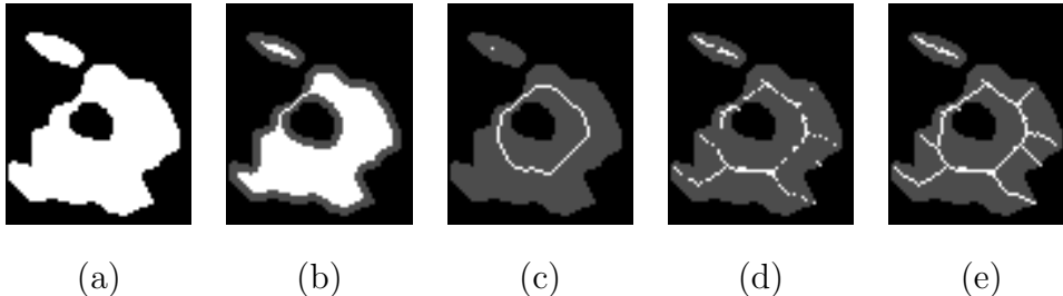
Fig. 2. (a): a set X (in white); (b): an homotopic thinning of X ; (c): ultimate homotopic skeleton of X ; (d): medial axis of X , computed by the algorithm of [25]; (e): ultimate homotopic skeleton of X constrained by the medial axis of X . In (b,c,d,e) the original set X appears in gray for comparison.
