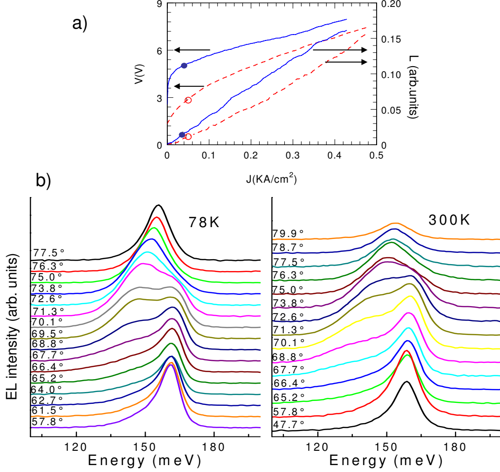
FIG. 3: a) Voltage and electroluminescence intensity as a function of the injected current density in pulsed operation (20 kHz, 500 ns) at 73.8° at 78 K (continuous line) and 300 K (dashed line). The dots indicate the working conditions for obtaining the electroluminescence spectra shown below. b) Electroluminescence spectra, offset each other for clarity, as functions of the propagating angle within the micro-cavity, at 78K and 5 V (left side) and at 300 K for an applied voltage of 2.8 V (right side). These voltages have been chosen as the lowest possible values to measure a spectrum at the two temperatures. In order to increase the electroluminescence signal, we worked at 50 % duty cycle (100 kHz repetition rate and 5 \mu s pulse width). Spectra are collected in step scan mode, with a spectral resolution of 16 cm -1 ; a f/1.5 ZnSe lens is used as collecting lens.
